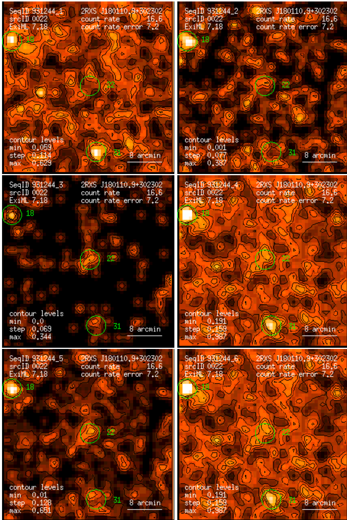
Figure 22: RASS 931244: detection 0022: band rate images, Gaussian filter: (1) PSPC channels 11 – 41, (2) 52 – 90, (3) 91 – 201, (4) 11 – 235, (5) 52 – 201, (6) 11 – 201. Broad band rates in counts/ks. Band rate contour levels in counts/ks/arcmin 2 .
