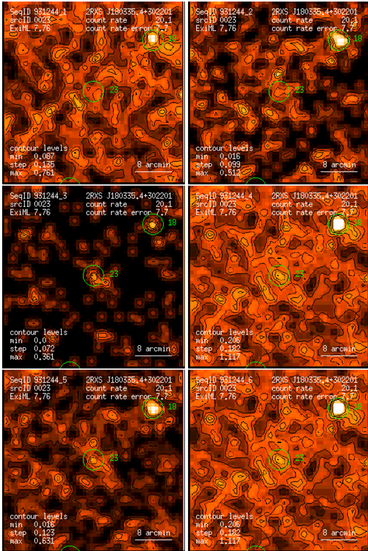
Figure 23: RASS 931244: detection 0023: band rate images, Gaussian filter: (1) PSPC channels 11 – 41, (2) 52 – 90, (3) 91 – 201, (4) 11 – 235, (5) 52 – 201, (6) 11 – 201. Broad band rates in counts/ks. Band rate contour levels in counts/ks/arcmin 2 .
