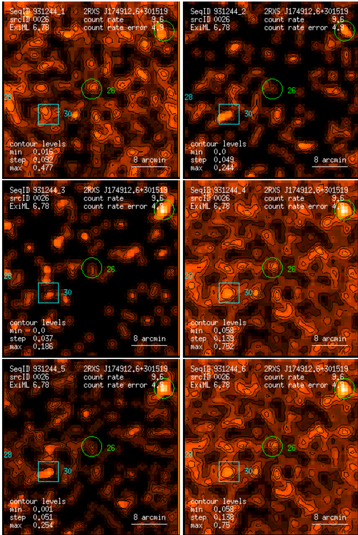
Figure 26: RASS 931244: detection 0026: band rate images, Gaussian filter: (1) PSPC channels 11 – 41, (2) 52 – 90, (3) 91 – 201, (4) 11 – 235, (5) 52 – 201, (6) 11 – 201. Broad band rates in counts/ks. Band rate contour levels in counts/ks/arcmin 2 .
