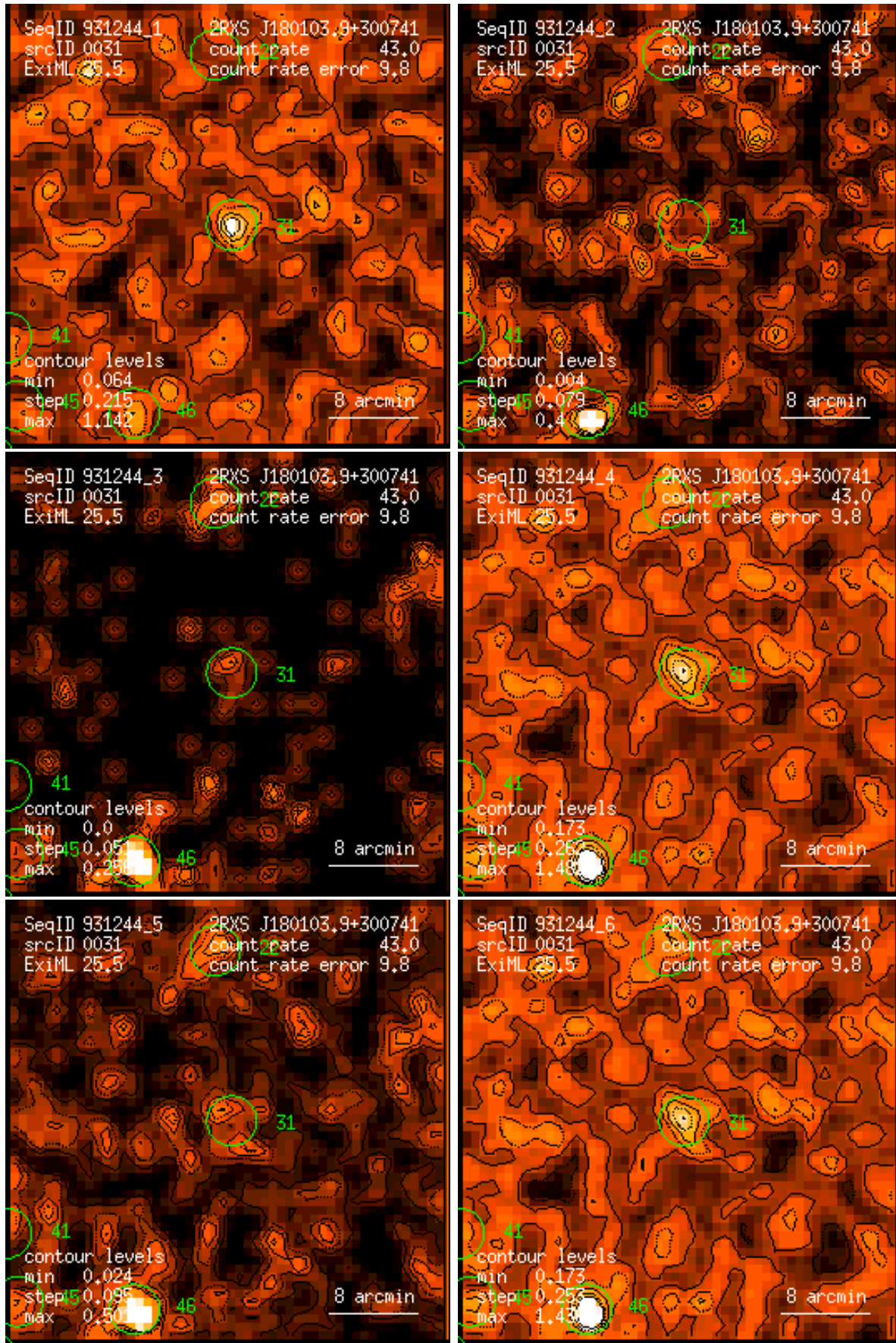
Figure 31: RASS 931244: detection 0031: band rate images, Gaussian filter: (1) PSPC channels 11 – 41, (2) 52 – 90, (3) 91 – 201, (4) 11 – 235, (5) 52 – 201, (6) 11 – 201. Broad band rates in counts/ks. Band rate contour levels in counts/ks/arcmin 2 .
