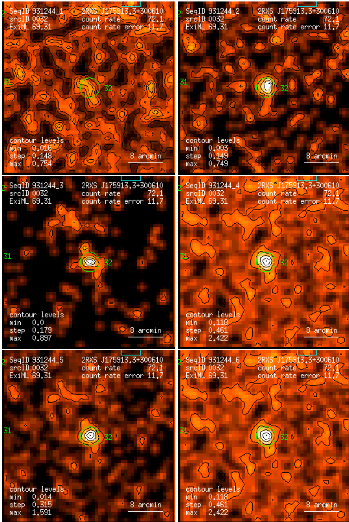
Figure 32: RASS 931244: detection 0032: band rate images, Gaussian filter: (1) PSPC channels 11 – 41, (2) 52 – 90, (3) 91 – 201, (4) 11 – 235, (5) 52 – 201, (6) 11 – 201. Broad band rates in counts/ks. Band rate contour levels in counts/ks/arcmin 2 .
