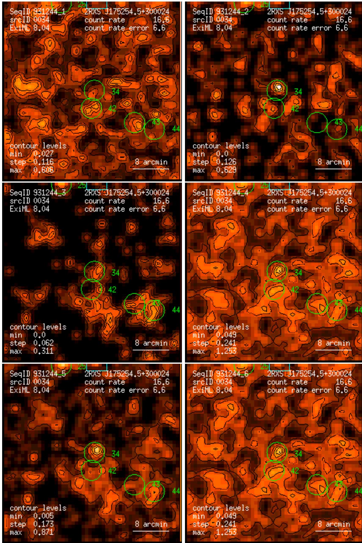
Figure 34: RASS 931244: detection 0034: band rate images, Gaussian filter: (1) PSPC channels 11 – 41, (2) 52 – 90, (3) 91 – 201, (4) 11 – 235, (5) 52 – 201, (6) 11 – 201. Broad band rates in counts/ks. Band rate contour levels in counts/ks/arcmin 2 .
