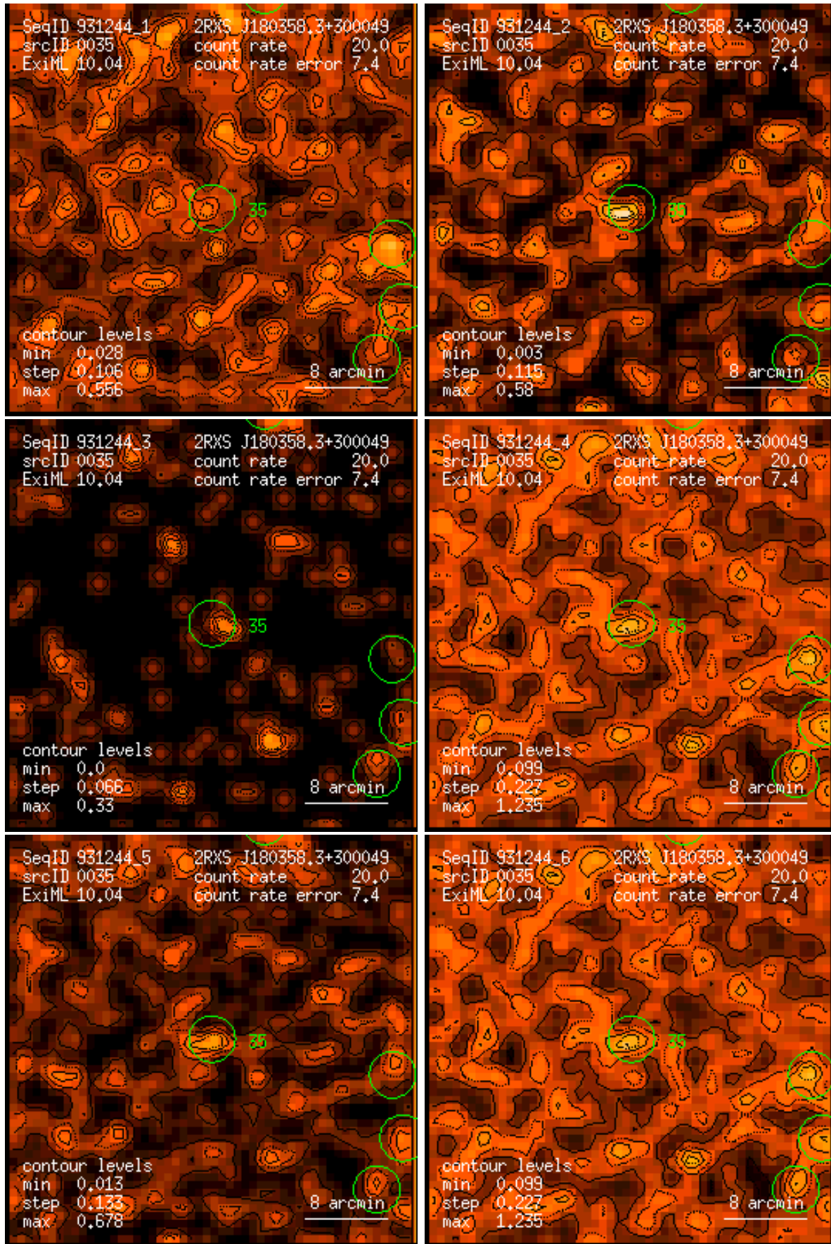
Figure 35: RASS 931244: detection 0035: band rate images, Gaussian filter: (1) PSPC channels 11 – 41, (2) 52 – 90, (3) 91 – 201, (4) 11 – 235, (5) 52 – 201, (6) 11 – 201. Broad band rates in counts/ks. Band rate contour levels in counts/ks/arcmin 2 .
