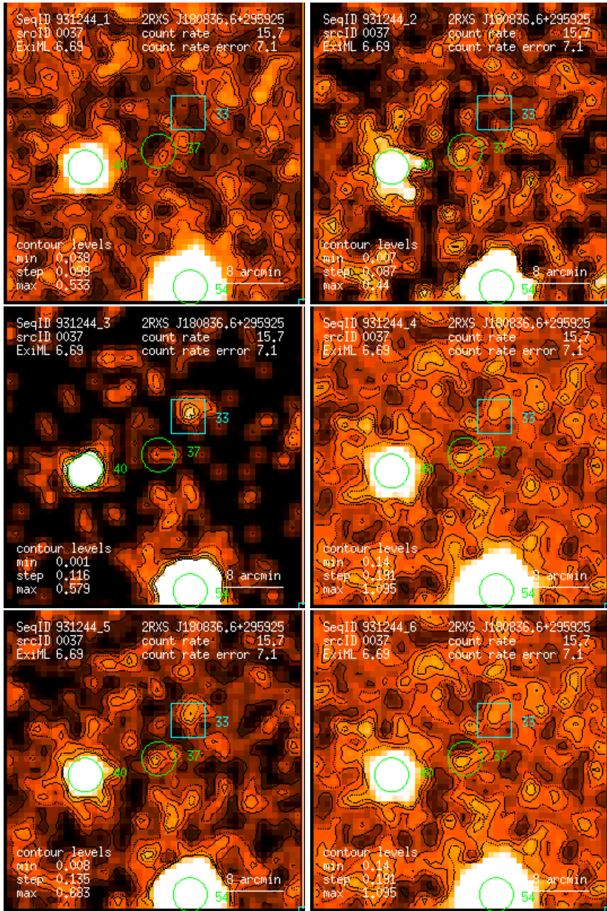
Figure 37: RASS 931244: detection 0037: band rate images, Gaussian filter: (1) PSPC channels 11 – 41, (2) 52 – 90, (3) 91 – 201, (4) 11 – 235, (5) 52 – 201, (6) 11 – 201. Broad band rates in counts/ks. Band rate contour levels in counts/ks/arcmin 2 .
