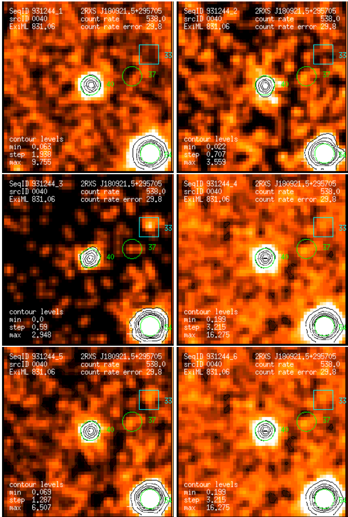
Figure 40: RASS 931244: detection 0040: band rate images, Gaussian filter: (1) PSPC channels 11 – 41, (2) 52 – 90, (3) 91 – 201, (4) 11 – 235, (5) 52 – 201, (6) 11 – 201. Broad band rates in counts/ks. Band rate contour levels in counts/ks/arcmin 2 .
