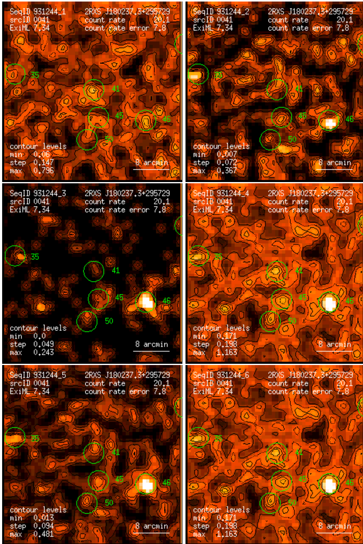
Figure 41: RASS 931244: detection 0041: band rate images, Gaussian filter: (1) PSPC channels 11 – 41, (2) 52 – 90, (3) 91 – 201, (4) 11 – 235, (5) 52 – 201, (6) 11 – 201. Broad band rates in counts/ks. Band rate contour levels in counts/ks/arcmin 2 .
