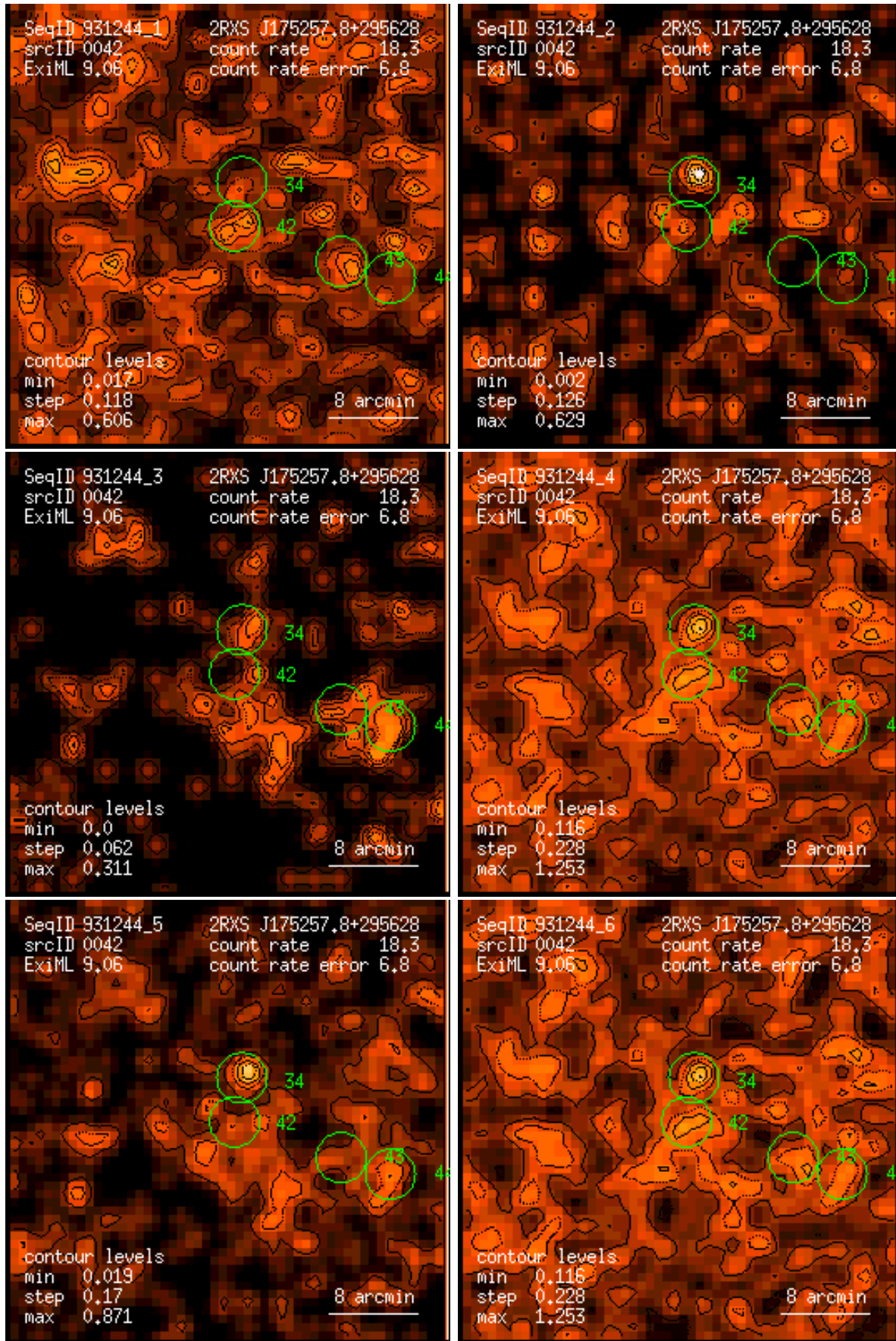
Figure 42: RASS 931244: detection 0042: band rate images, Gaussian filter: (1) PSPC channels 11 – 41, (2) 52 – 90, (3) 91 – 201, (4) 11 – 235, (5) 52 – 201, (6) 11 – 201. Broad band rates in counts/ks. Band rate contour levels in counts/ks/arcmin 2 .
