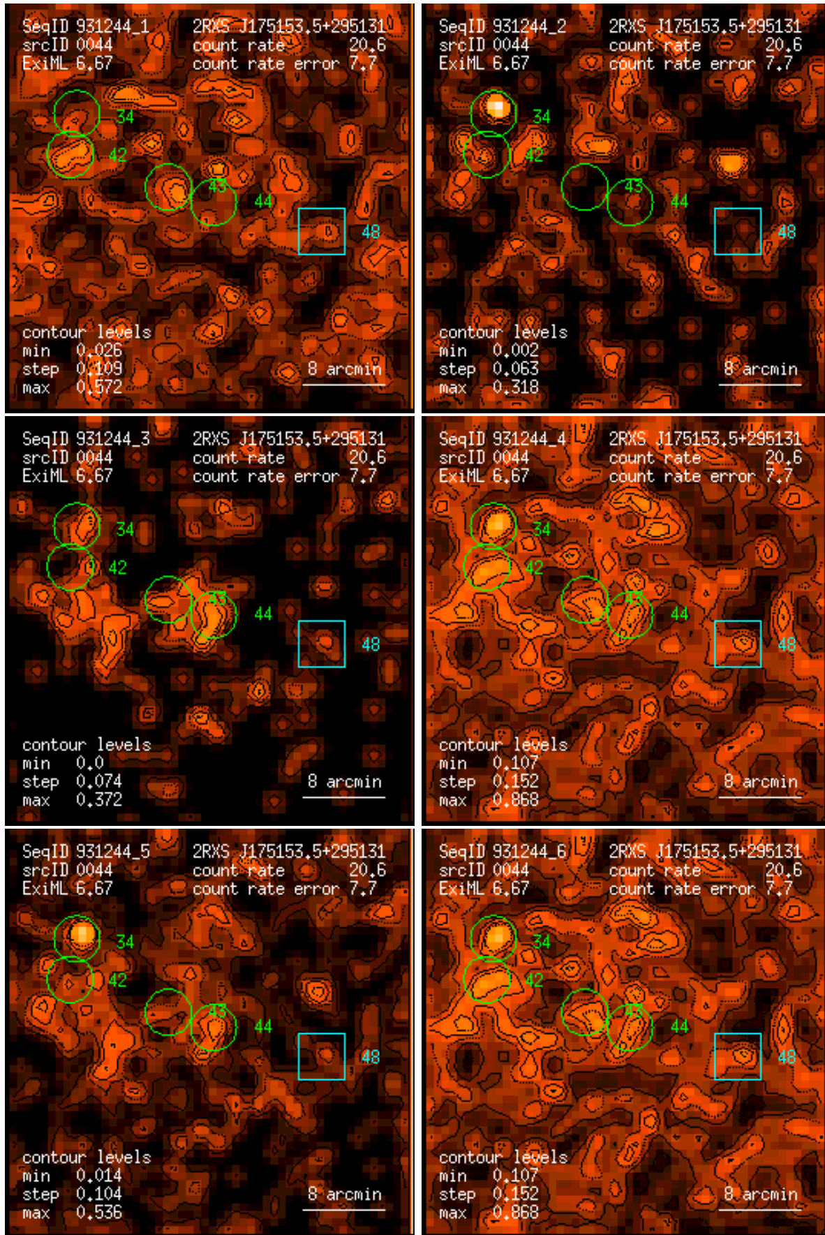
Figure 44: RASS 931244: detection 0044: band rate images, Gaussian filter: (1) PSPC channels 11 – 41, (2) 52 – 90, (3) 91 – 201, (4) 11 – 235, (5) 52 – 201, (6) 11 – 201. Broad band rates in counts/ks. Band rate contour levels in counts/ks/arcmin 2 .
