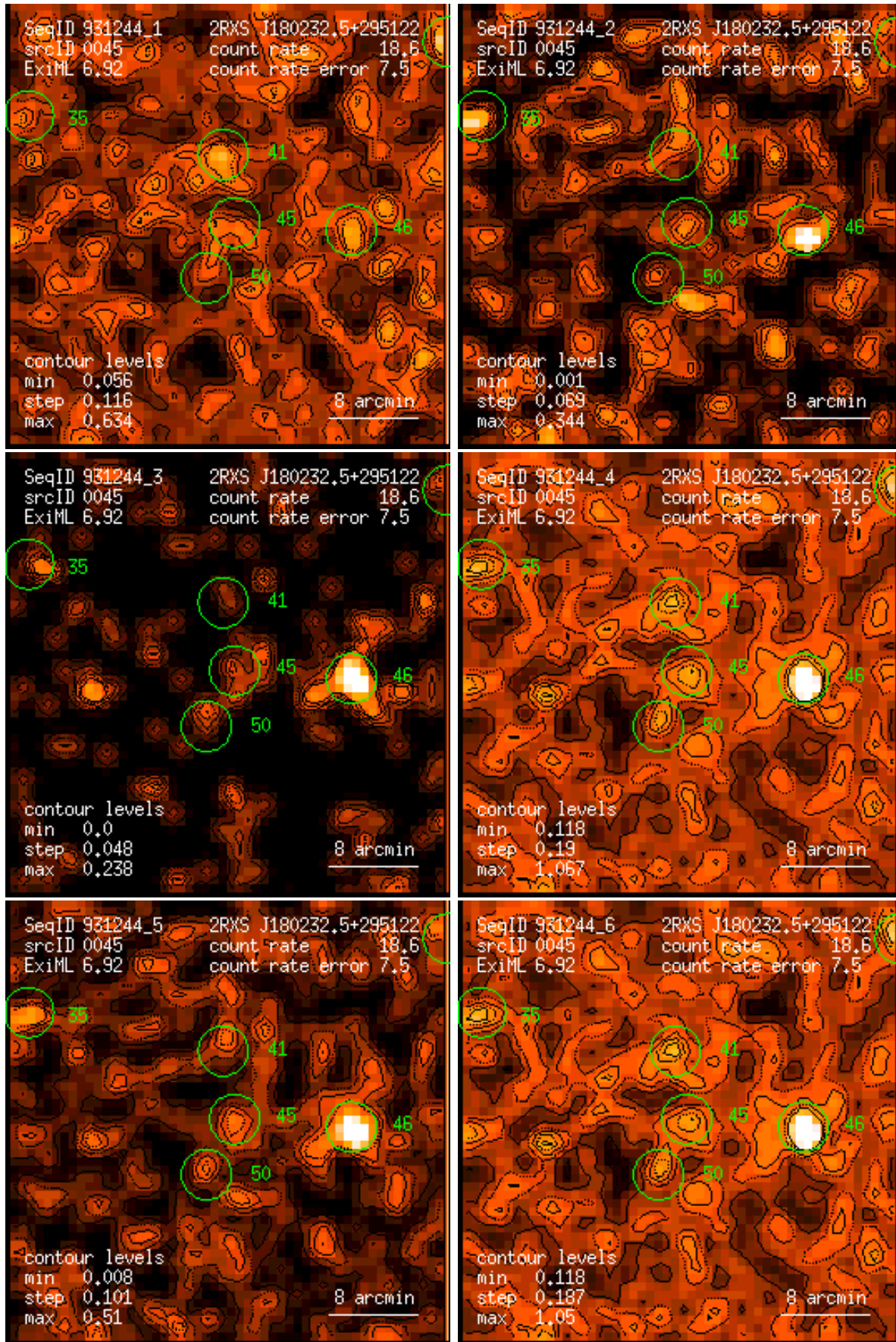
Figure 45: RASS 931244: detection 0045: band rate images, Gaussian filter: (1) PSPC channels 11 – 41, (2) 52 – 90, (3) 91 – 201, (4) 11 – 235, (5) 52 – 201, (6) 11 – 201. Broad band rates in counts/ks. Band rate contour levels in counts/ks/arcmin 2 .
