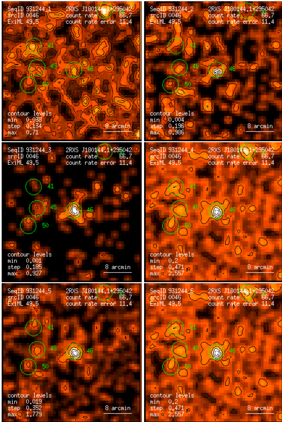
Figure 46: RASS 931244: detection 0046: band rate images, Gaussian filter: (1) PSPC channels 11 – 41, (2) 52 – 90, (3) 91 – 201, (4) 11 – 235, (5) 52 – 201, (6) 11 – 201. Broad band rates in counts/ks. Band rate contour levels in counts/ks/arcmin 2 .
