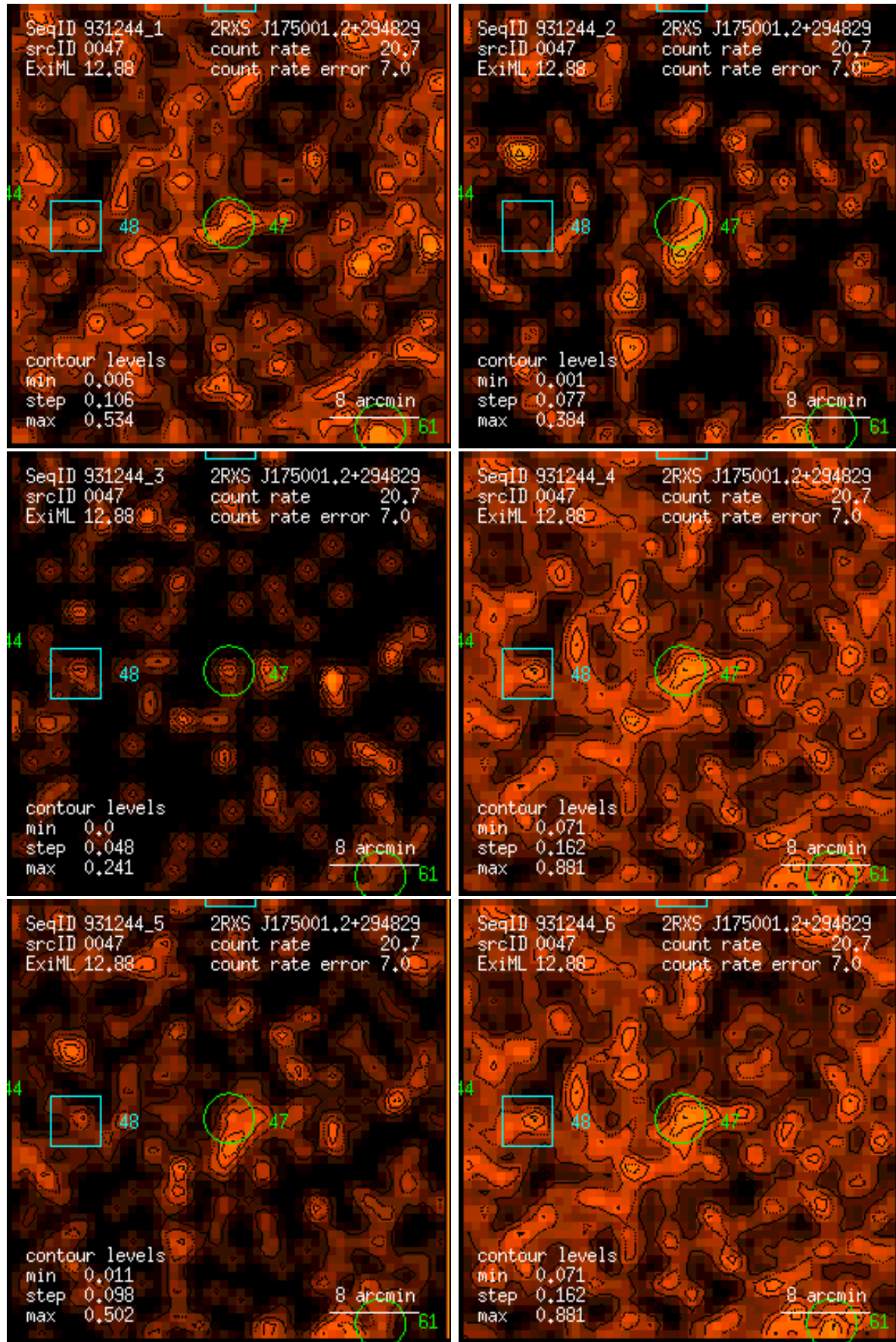
Figure 47: RASS 931244: detection 0047: band rate images, Gaussian filter: (1) PSPC channels 11 – 41, (2) 52 – 90, (3) 91 – 201, (4) 11 – 235, (5) 52 – 201, (6) 11 – 201. Broad band rates in counts/ks. Band rate contour levels in counts/ks/arcmin 2 .
