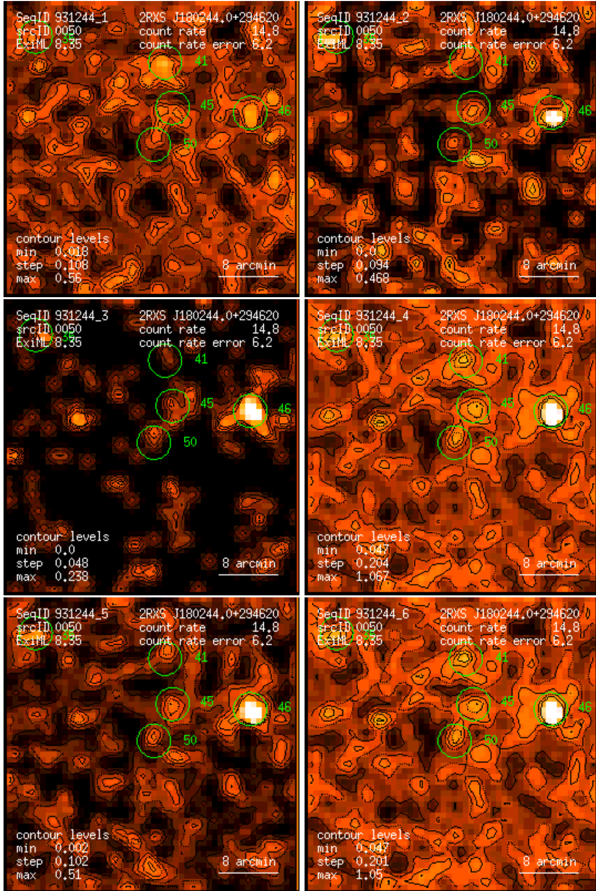
Figure 50: RASS 931244: detection 0050: band rate images, Gaussian filter: (1) PSPC channels 11 – 41, (2) 52 – 90, (3) 91 – 201, (4) 11 – 235, (5) 52 – 201, (6) 11 – 201. Broad band rates in counts/ks. Band rate contour levels in counts/ks/arcmin 2 .
