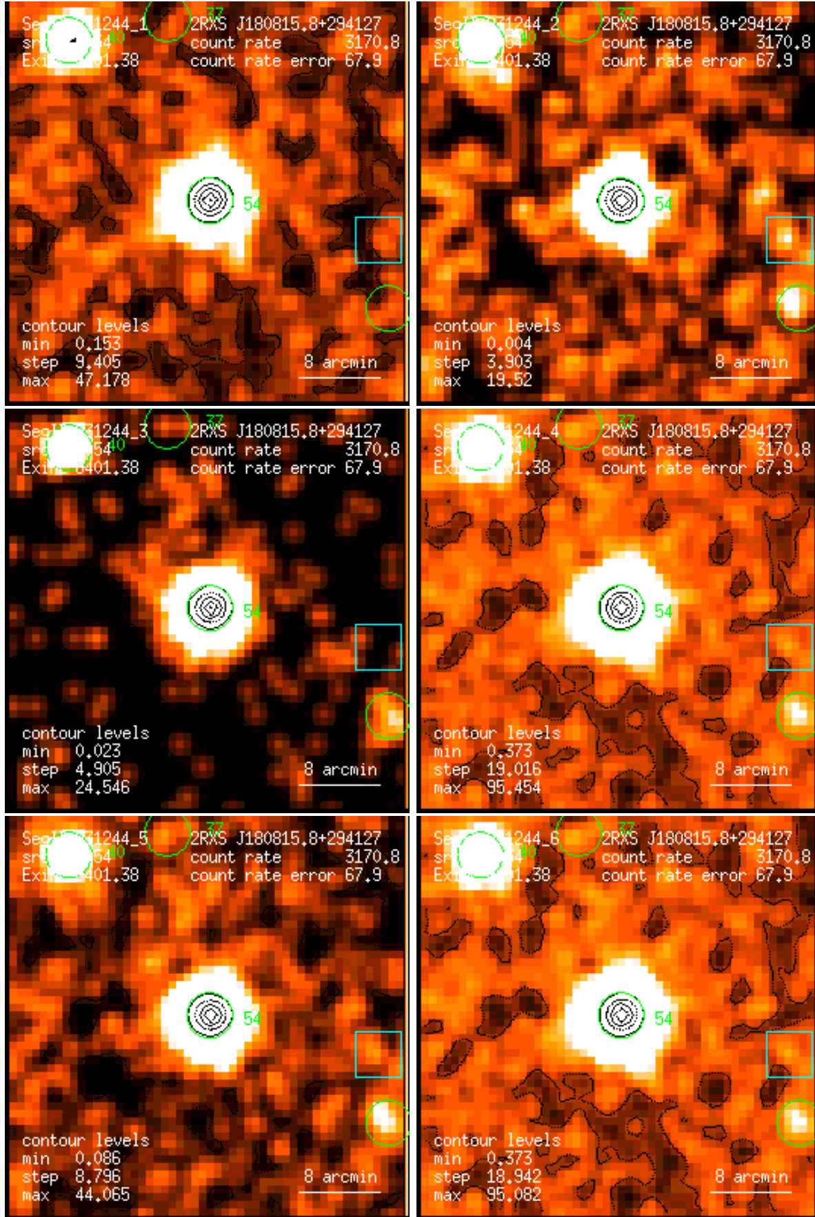
Figure 54: RASS 931244: detection 0054: band rate images, Gaussian filter: (1) PSPC channels 11 – 41, (2) 52 – 90, (3) 91 – 201, (4) 11 – 235, (5) 52 – 201, (6) 11 – 201. Broad band rates in counts/ks. Band rate contour levels in counts/ks/arcmin 2 .
