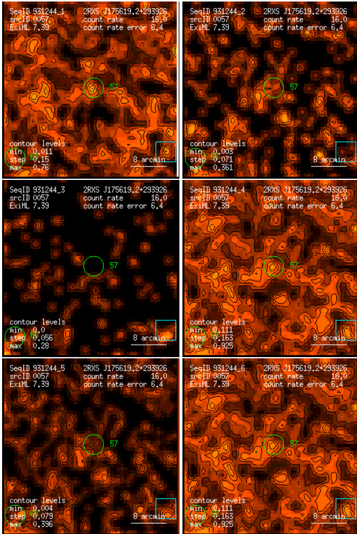
Figure 57: RASS 931244: detection 0057: band rate images, Gaussian filter: (1) PSPC channels 11 – 41, (2) 52 – 90, (3) 91 – 201, (4) 11 – 235, (5) 52 – 201, (6) 11 – 201. Broad band rates in counts/ks. Band rate contour levels in counts/ks/arcmin 2 .
