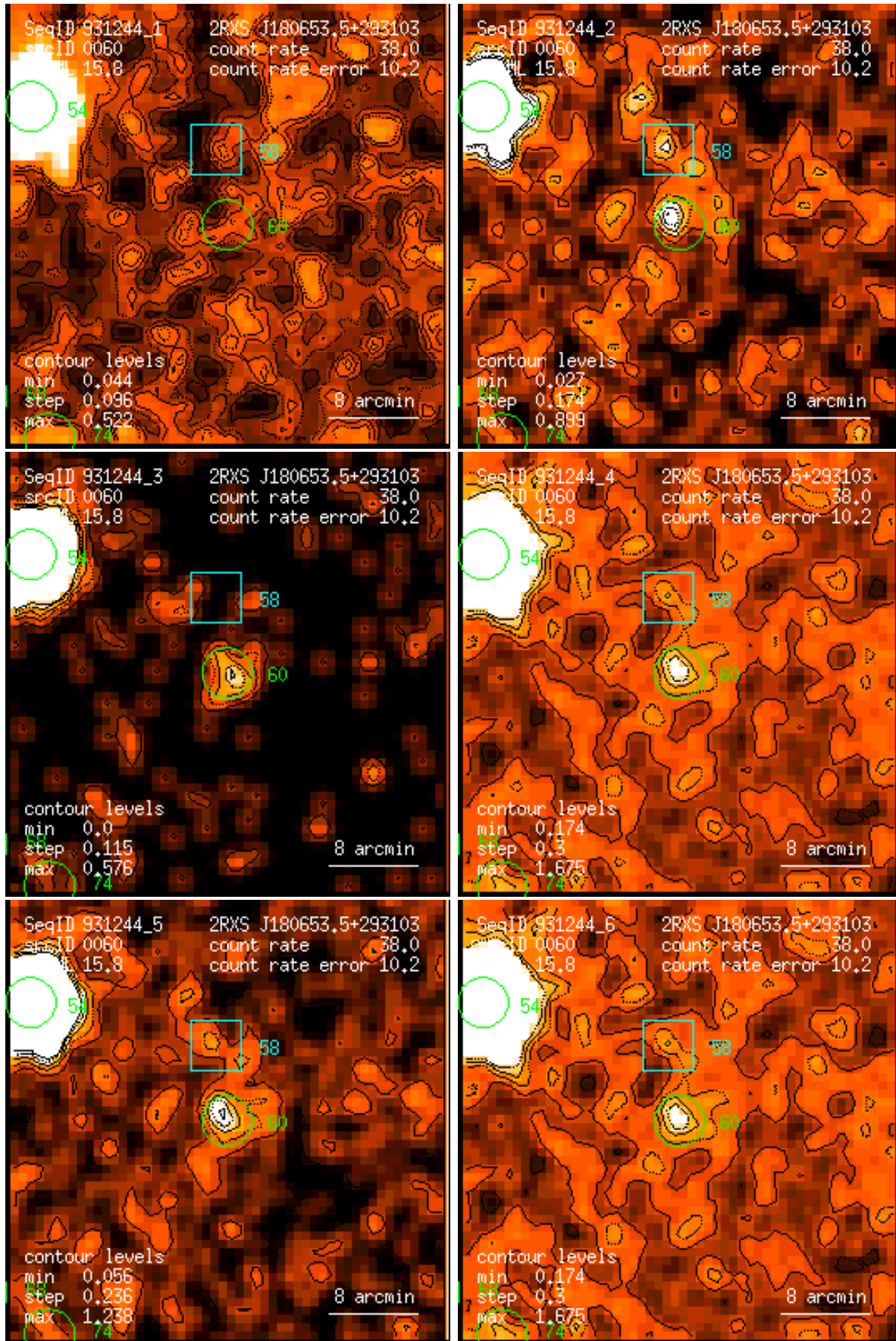
Figure 60: RASS 931244: detection 0060: band rate images, Gaussian filter: (1) PSPC channels 11 – 41, (2) 52 – 90, (3) 91 – 201, (4) 11 – 235, (5) 52 – 201, (6) 11 – 201. Broad band rates in counts/ks. Band rate contour levels in counts/ks/arcmin 2 .
