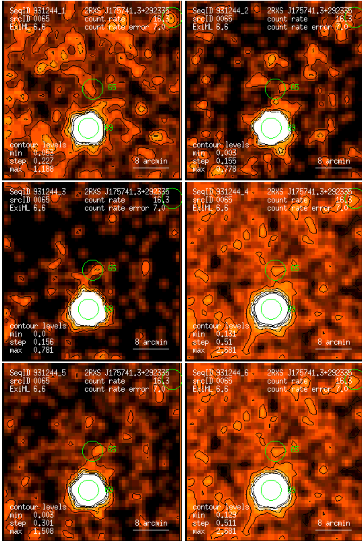
Figure 65: RASS 931244: detection 0065: band rate images, Gaussian filter: (1) PSPC channels 11 – 41, (2) 52 – 90, (3) 91 – 201, (4) 11 – 235, (5) 52 – 201, (6) 11 – 201. Broad band rates in counts/ks. Band rate contour levels in counts/ks/arcmin 2 .
