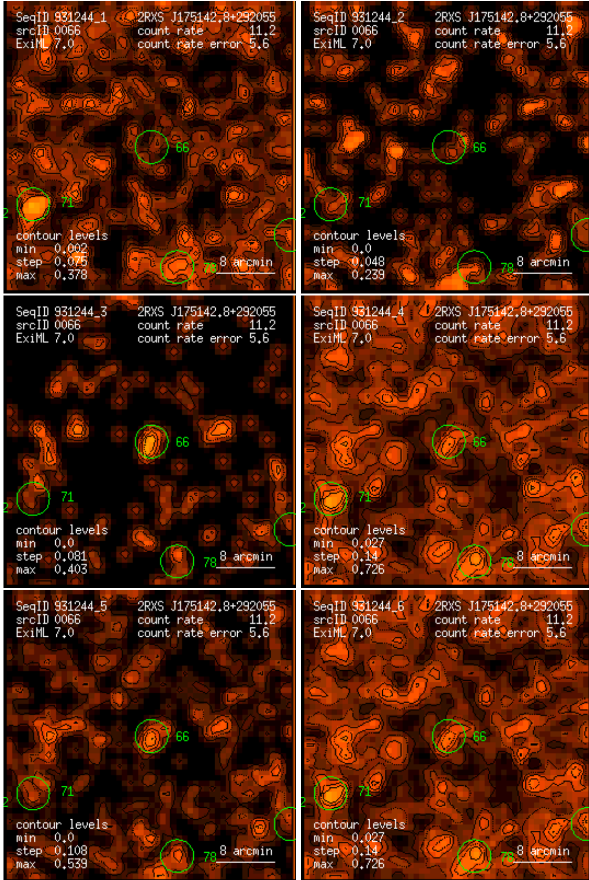
Figure 66: RASS 931244: detection 0066: band rate images, Gaussian filter: (1) PSPC channels 11 – 41, (2) 52 – 90, (3) 91 – 201, (4) 11 – 235, (5) 52 – 201, (6) 11 – 201. Broad band rates in counts/ks. Band rate contour levels in counts/ks/arcmin 2 .
