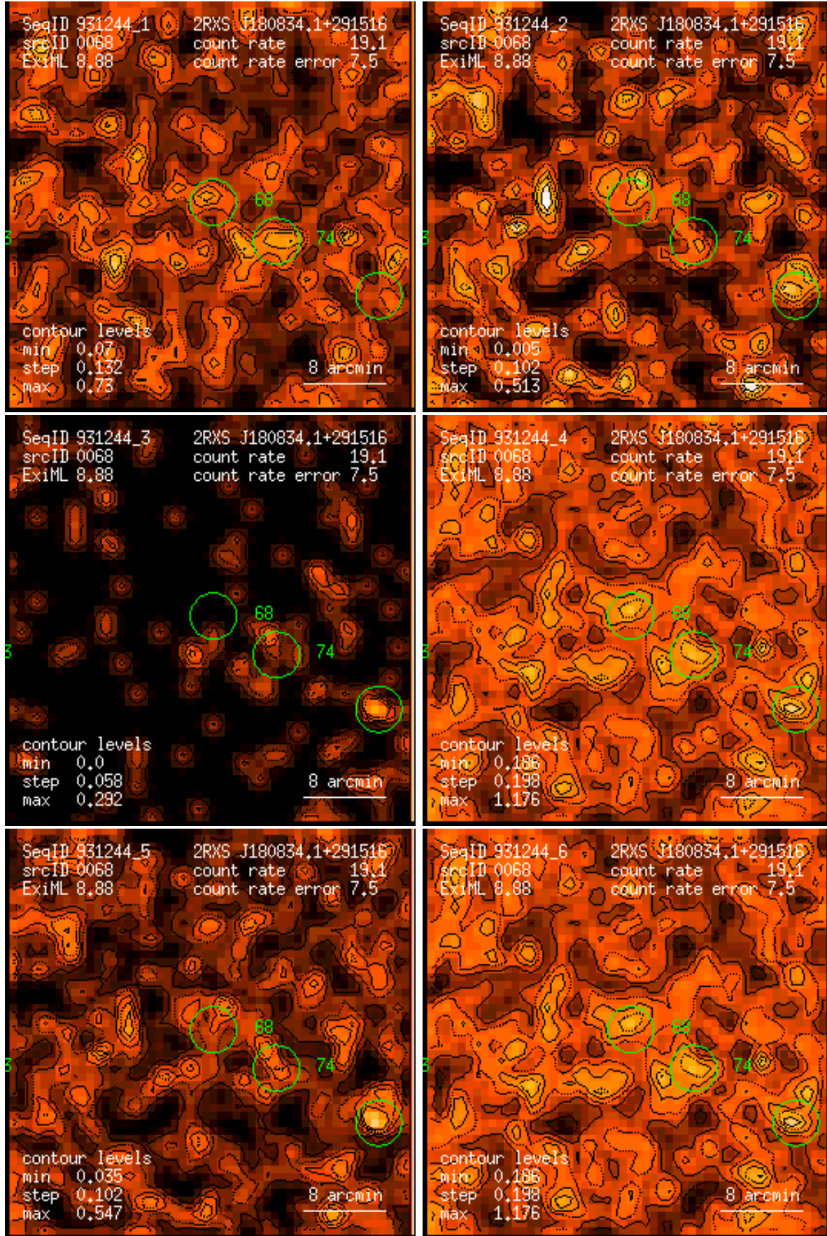
Figure 68: RASS 931244: detection 0068: band rate images, Gaussian filter: (1) PSPC channels 11 – 41, (2) 52 – 90, (3) 91 – 201, (4) 11 – 235, (5) 52 – 201, (6) 11 – 201. Broad band rates in counts/ks. Band rate contour levels in counts/ks/arcmin 2 .
