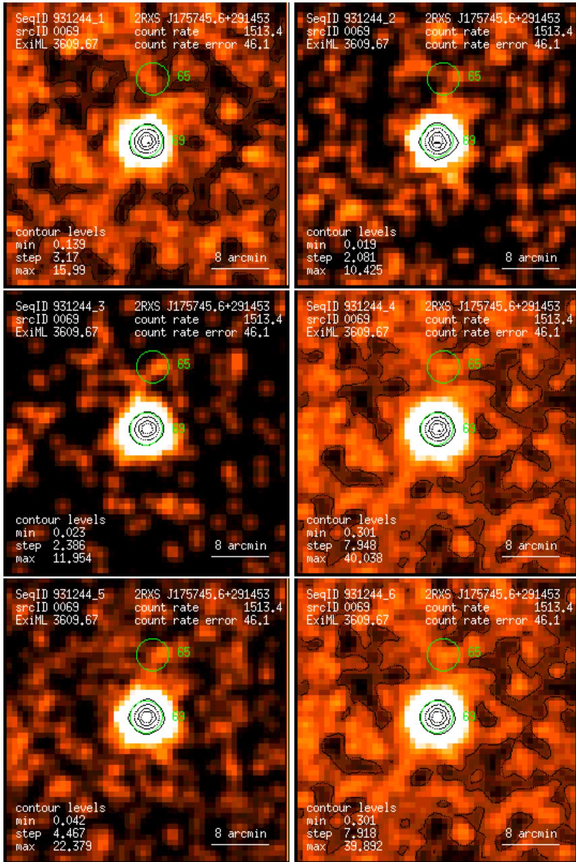
Figure 69: RASS 931244: detection 0069: band rate images, Gaussian filter: (1) PSPC channels 11 – 41, (2) 52 – 90, (3) 91 – 201, (4) 11 – 235, (5) 52 – 201, (6) 11 – 201. Broad band rates in counts/ks. Band rate contour levels in counts/ks/arcmin 2 .
