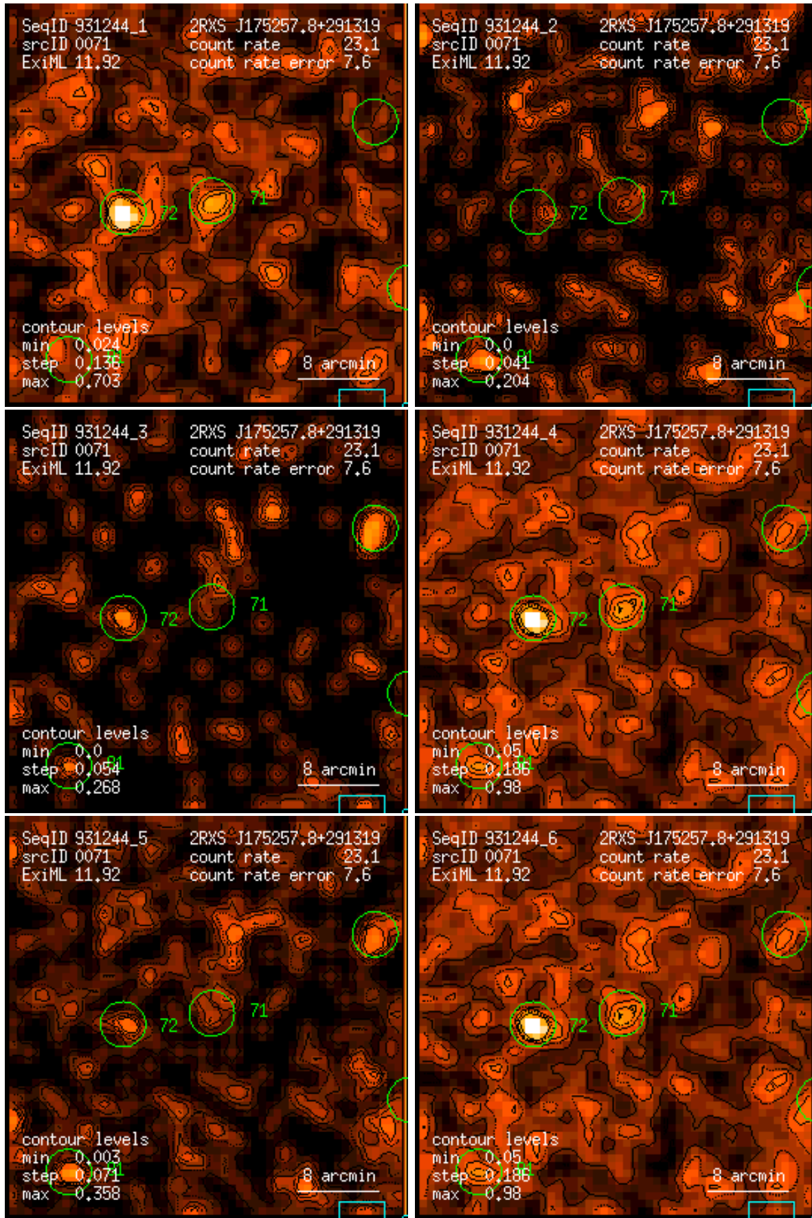
Figure 71: RASS 931244: detection 0071: band rate images, Gaussian filter: (1) PSPC channels 11 – 41, (2) 52 – 90, (3) 91 – 201, (4) 11 – 235, (5) 52 – 201, (6) 11 – 201. Broad band rates in counts/ks. Band rate contour levels in counts/ks/arcmin 2 .
