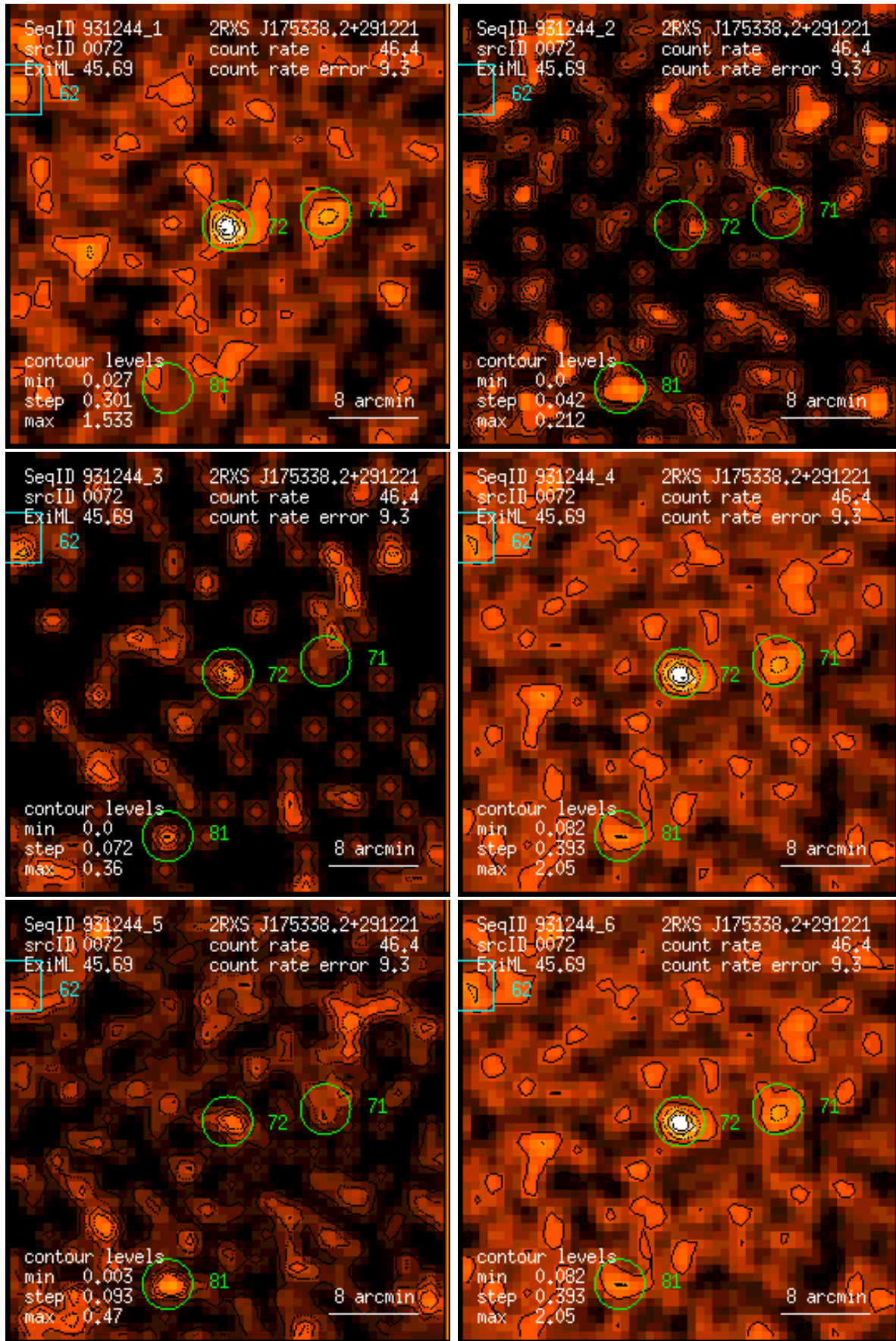
Figure 72: RASS 931244: detection 0072: band rate images, Gaussian filter: (1) PSPC channels 11 – 41, (2) 52 – 90, (3) 91 – 201, (4) 11 – 235, (5) 52 – 201, (6) 11 – 201. Broad band rates in counts/ks. Band rate contour levels in counts/ks/arcmin 2 .
