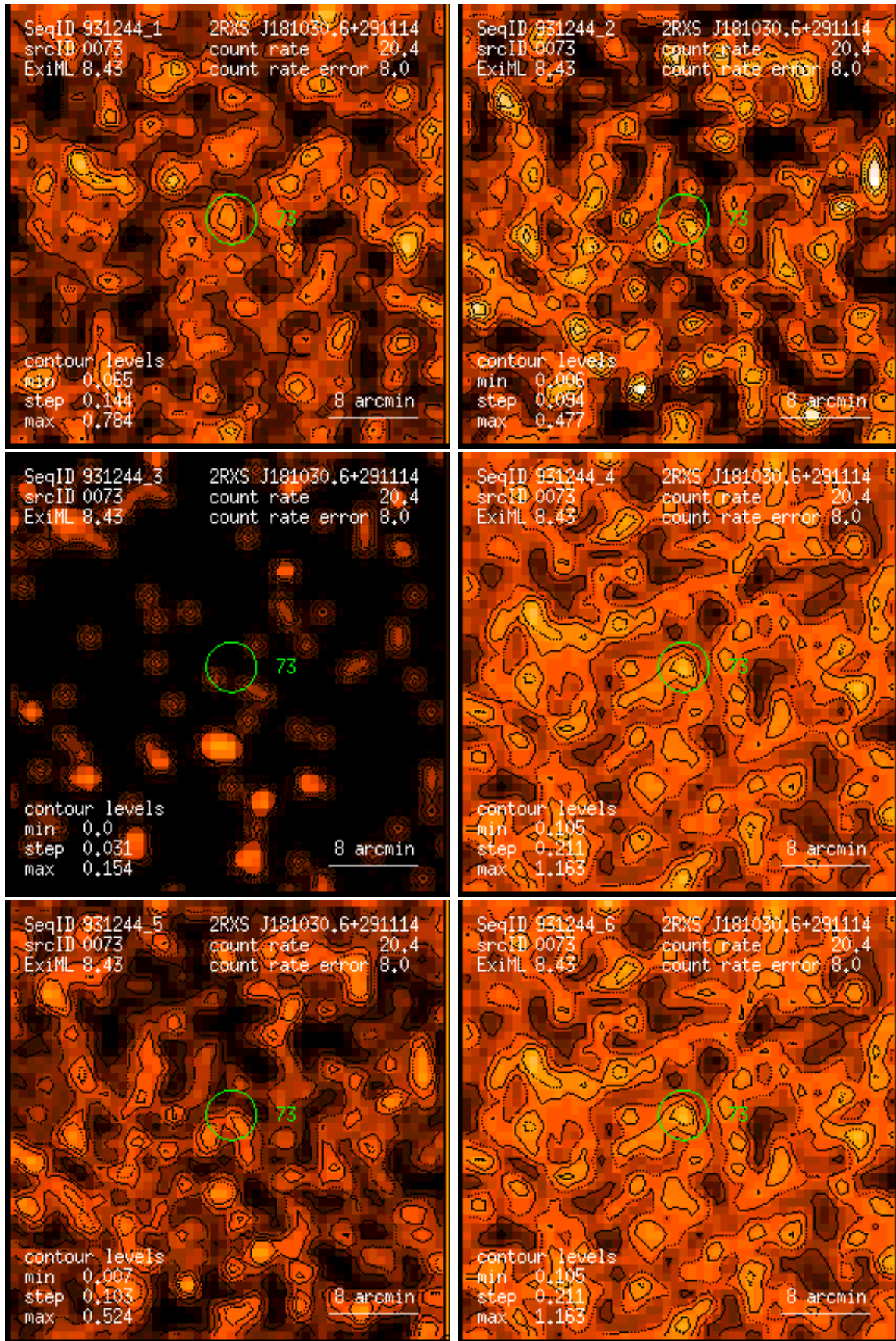
Figure 73: RASS 931244: detection 0073: band rate images, Gaussian filter: (1) PSPC channels 11 – 41, (2) 52 – 90, (3) 91 – 201, (4) 11 – 235, (5) 52 – 201, (6) 11 – 201. Broad band rates in counts/ks. Band rate contour levels in counts/ks/arcmin 2 .
