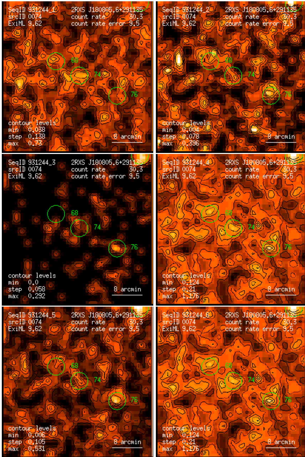
Figure 74: RASS 931244: detection 0074: band rate images, Gaussian filter: (1) PSPC channels 11 – 41, (2) 52 – 90, (3) 91 – 201, (4) 11 – 235, (5) 52 – 201, (6) 11 – 201. Broad band rates in counts/ks. Band rate contour levels in counts/ks/arcmin 2 .
