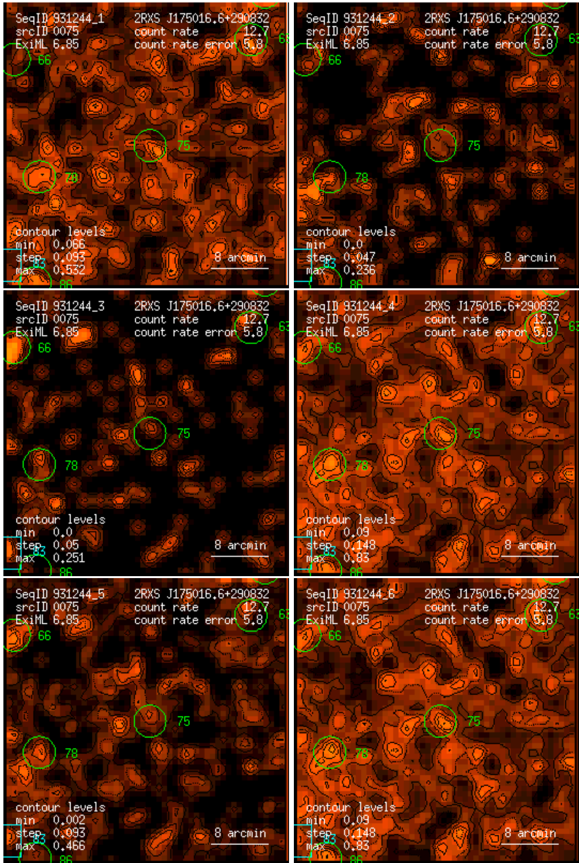
Figure 75: RASS 931244: detection 0075: band rate images, Gaussian filter: (1) PSPC channels 11 – 41, (2) 52 – 90, (3) 91 – 201, (4) 11 – 235, (5) 52 – 201, (6) 11 – 201. Broad band rates in counts/ks. Band rate contour levels in counts/ks/arcmin 2 .
