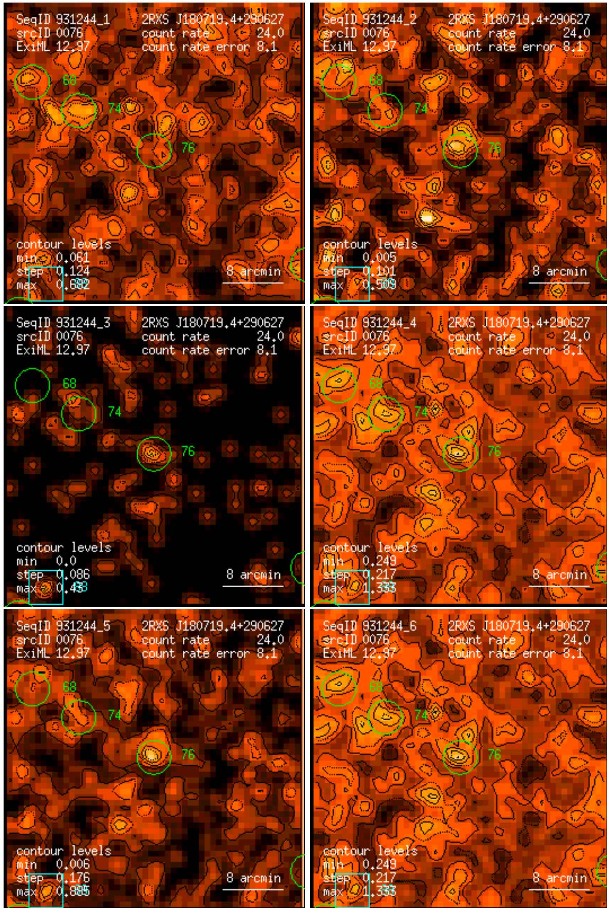
Figure 76: RASS 931244: detection 0076: band rate images, Gaussian filter: (1) PSPC channels 11 – 41, (2) 52 – 90, (3) 91 – 201, (4) 11 – 235, (5) 52 – 201, (6) 11 – 201. Broad band rates in counts/ks. Band rate contour levels in counts/ks/arcmin 2 .
