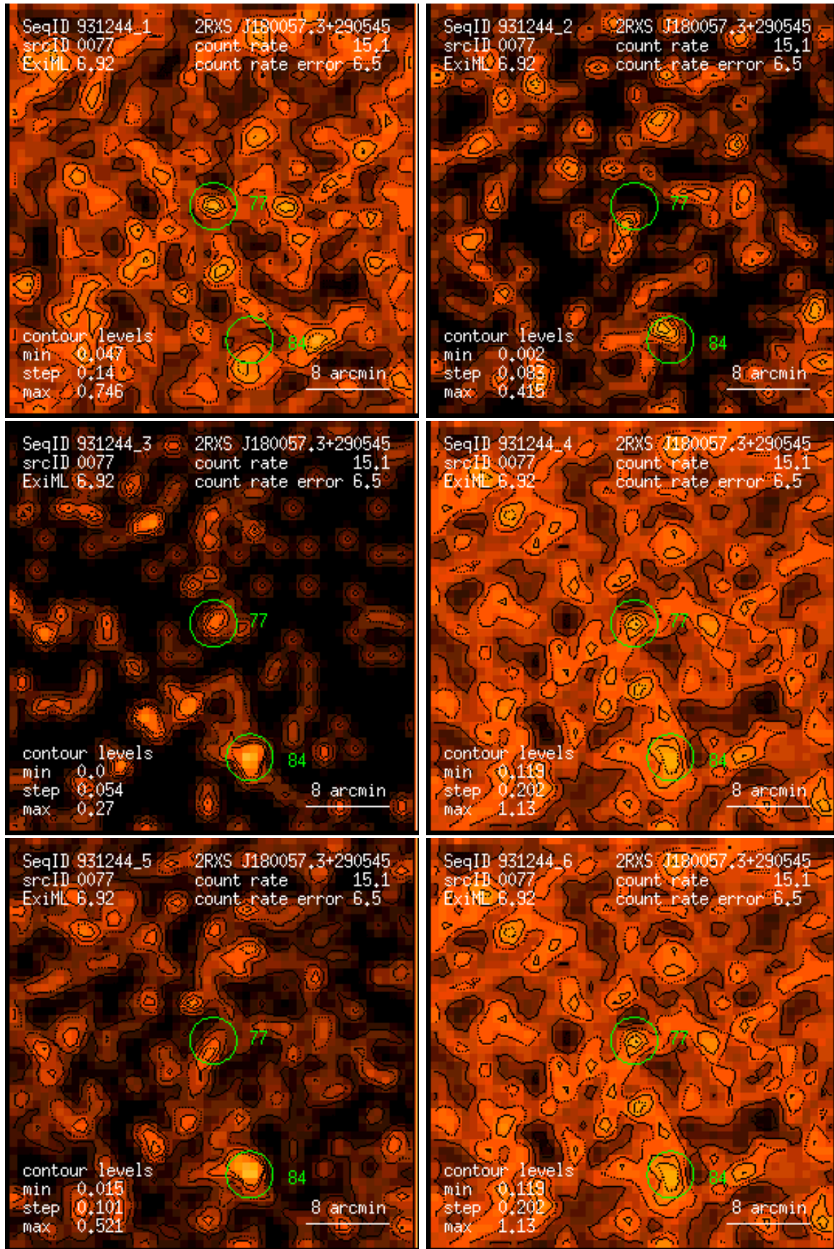
Figure 77: RASS 931244: detection 0077: band rate images, Gaussian filter: (1) PSPC channels 11 – 41, (2) 52 – 90, (3) 91 – 201, (4) 11 – 235, (5) 52 – 201, (6) 11 – 201. Broad band rates in counts/ks. Band rate contour levels in counts/ks/arcmin 2 .
