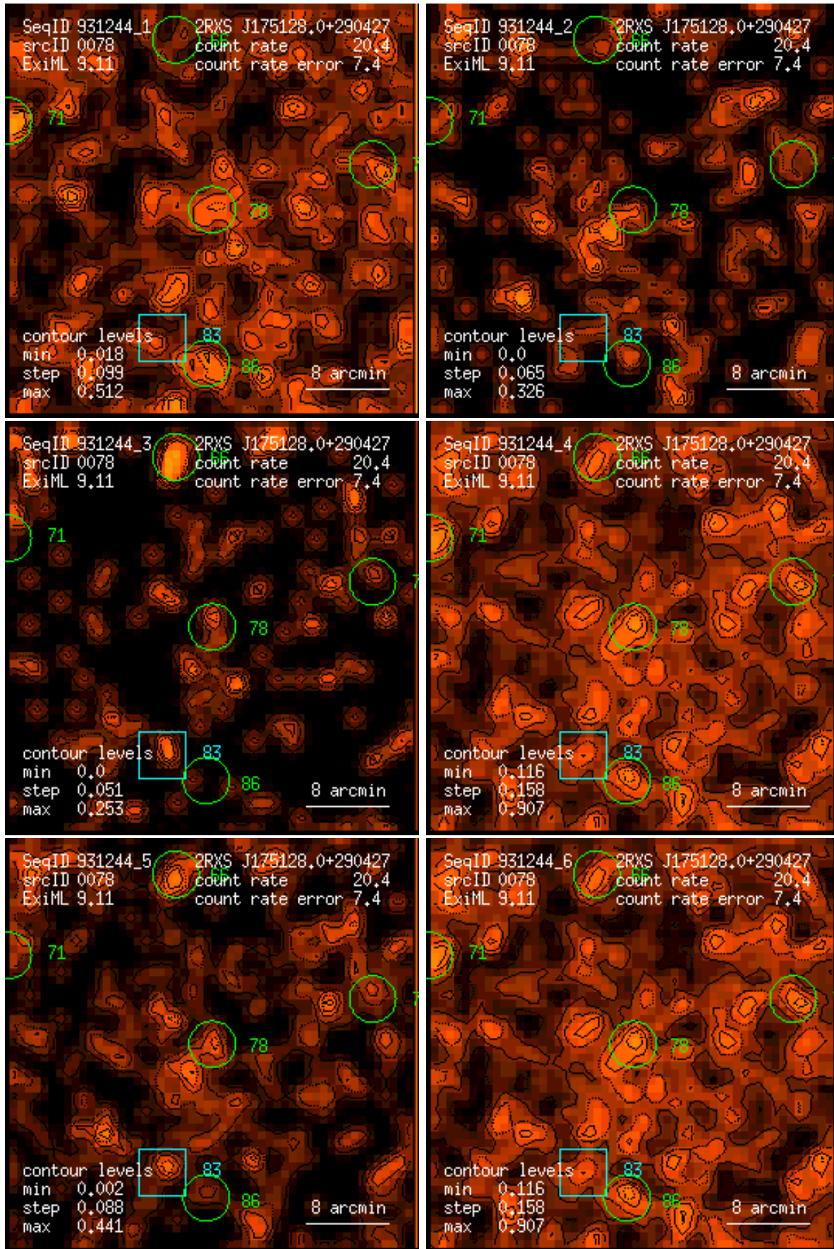
Figure 78: RASS 931244: detection 0078: band rate images, Gaussian filter: (1) PSPC channels 11 – 41, (2) 52 – 90, (3) 91 – 201, (4) 11 – 235, (5) 52 – 201, (6) 11 – 201. Broad band rates in counts/ks. Band rate contour levels in counts/ks/arcmin 2 .
