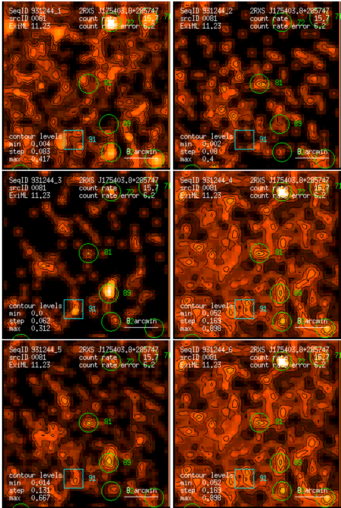
Figure 81: RASS 931244: detection 0081: band rate images, Gaussian filter: (1) PSPC channels 11 – 41, (2) 52 – 90, (3) 91 – 201, (4) 11 – 235, (5) 52 – 201, (6) 11 – 201. Broad band rates in counts/ks. Band rate contour levels in counts/ks/arcmin 2 .
