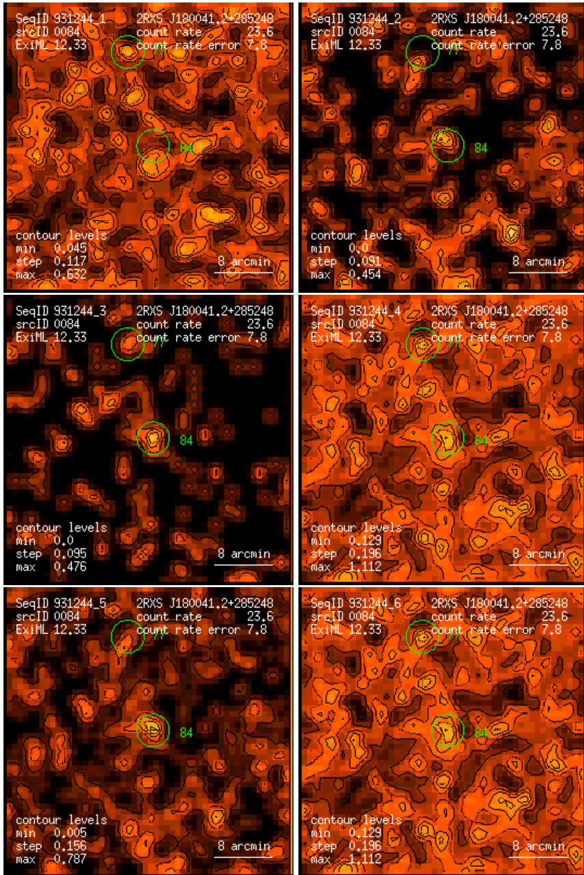
Figure 84: RASS 931244: detection 0084: band rate images, Gaussian filter: (1) PSPC channels 11 – 41, (2) 52 – 90, (3) 91 – 201, (4) 11 – 235, (5) 52 – 201, (6) 11 – 201. Broad band rates in counts/ks. Band rate contour levels in counts/ks/arcmin 2 .
