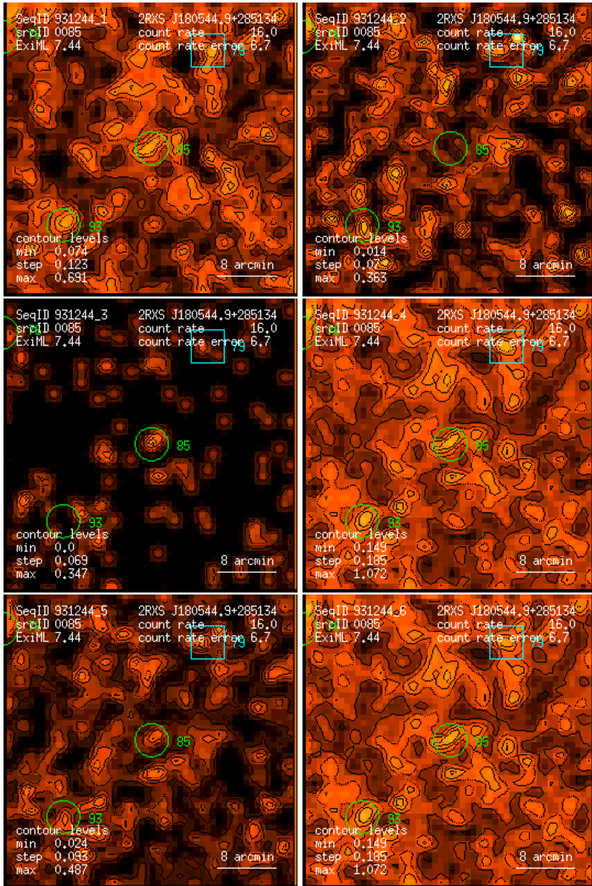
Figure 85: RASS 931244: detection 0085: band rate images, Gaussian filter: (1) PSPC channels 11 – 41, (2) 52 – 90, (3) 91 – 201, (4) 11 – 235, (5) 52 – 201, (6) 11 – 201. Broad band rates in counts/ks. Band rate contour levels in counts/ks/arcmin 2 .
