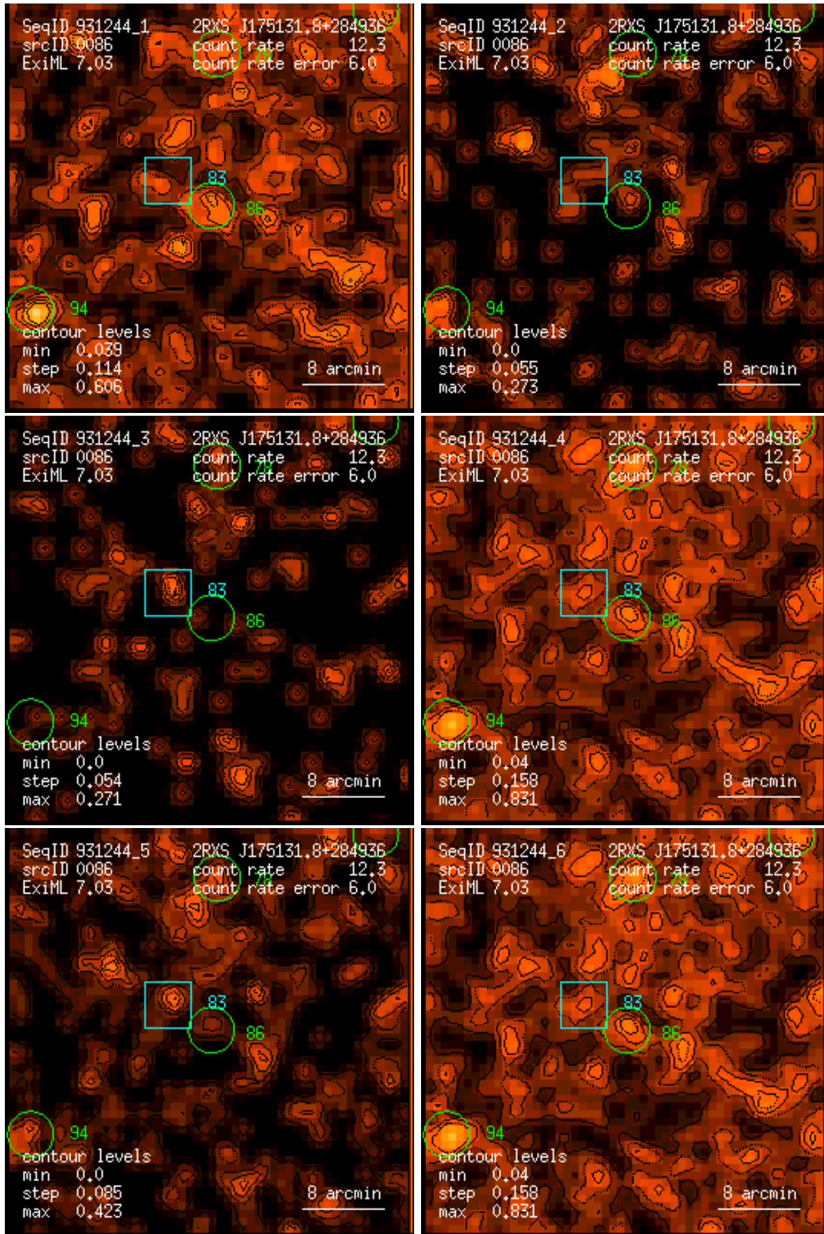
Figure 86: RASS 931244: detection 0086: band rate images, Gaussian filter: (1) PSPC channels 11 – 41, (2) 52 – 90, (3) 91 – 201, (4) 11 – 235, (5) 52 – 201, (6) 11 – 201. Broad band rates in counts/ks. Band rate contour levels in counts/ks/arcmin 2 .
