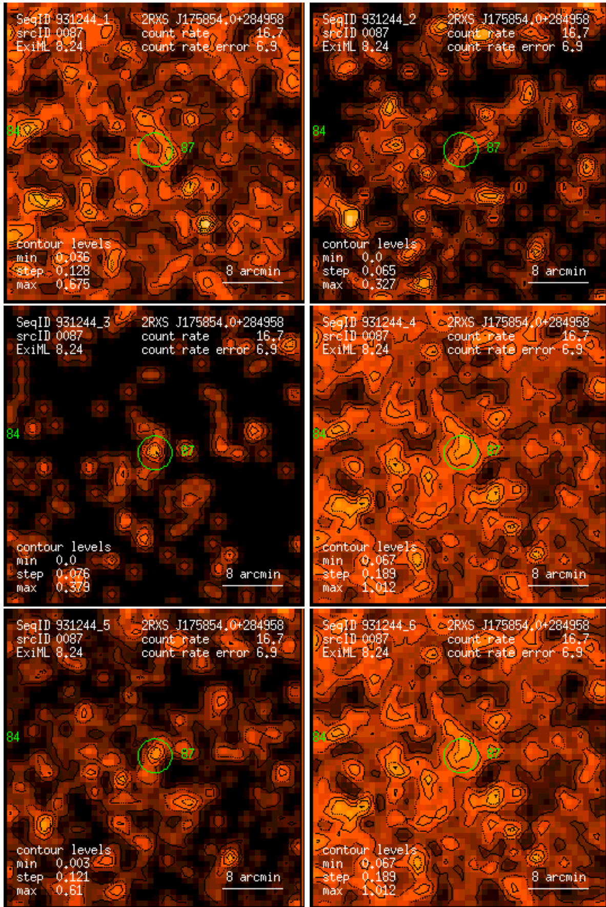
Figure 87: RASS 931244: detection 0087: band rate images, Gaussian filter: (1) PSPC channels 11 – 41, (2) 52 – 90, (3) 91 – 201, (4) 11 – 235, (5) 52 – 201, (6) 11 – 201. Broad band rates in counts/ks. Band rate contour levels in counts/ks/arcmin 2 .
