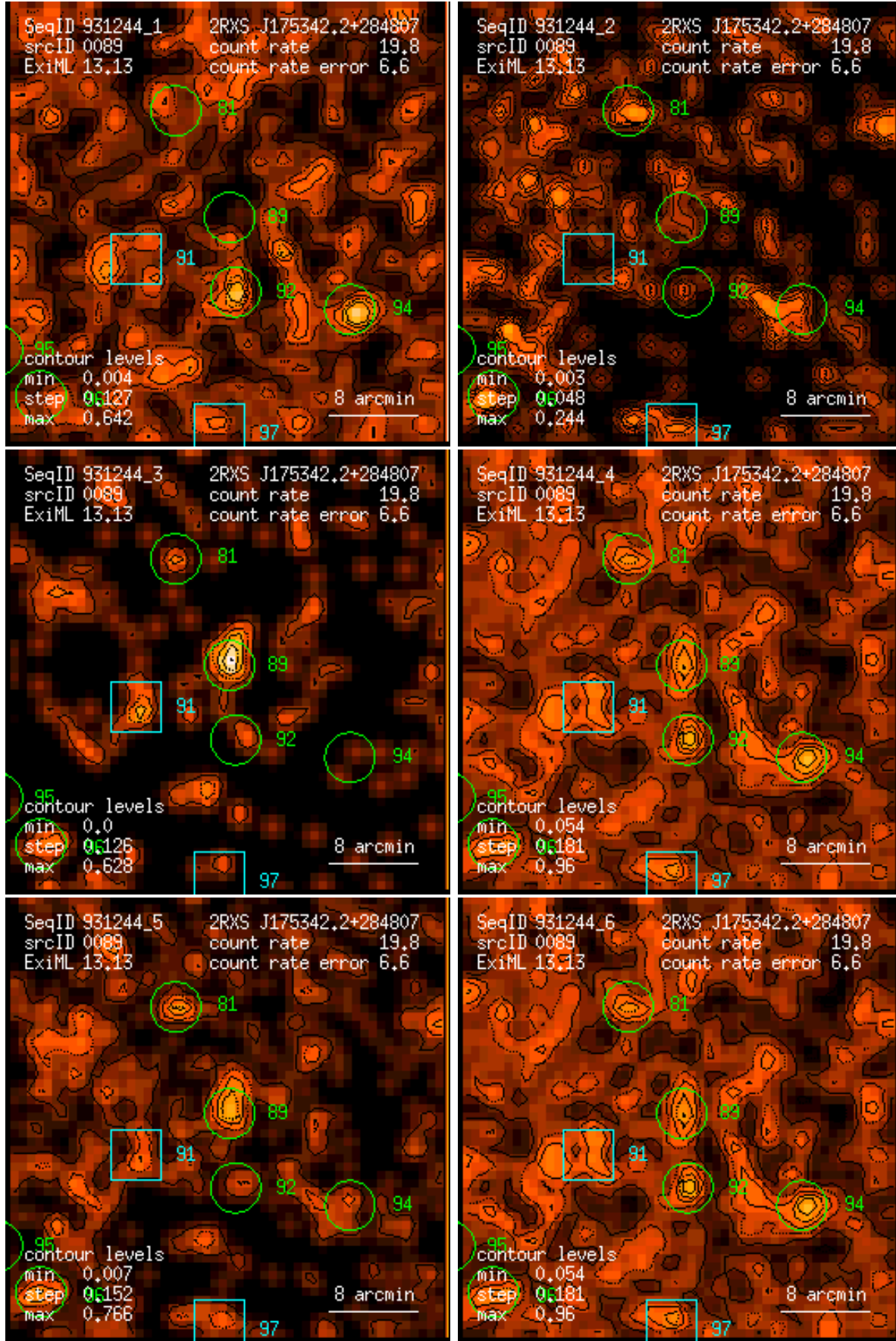
Figure 89: RASS 931244: detection 0089: band rate images, Gaussian filter: (1) PSPC channels 11 – 41, (2) 52 – 90, (3) 91 – 201, (4) 11 – 235, (5) 52 – 201, (6) 11 – 201. Broad band rates in counts/ks. Band rate contour levels in counts/ks/arcmin 2 .
