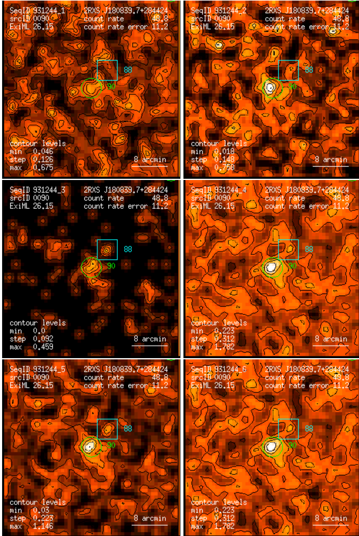
Figure 90: RASS 931244: detection 0090: band rate images, Gaussian filter: (1) PSPC channels 11 – 41, (2) 52 – 90, (3) 91 – 201, (4) 11 – 235, (5) 52 – 201, (6) 11 – 201. Broad band rates in counts/ks. Band rate contour levels in counts/ks/arcmin 2 .
