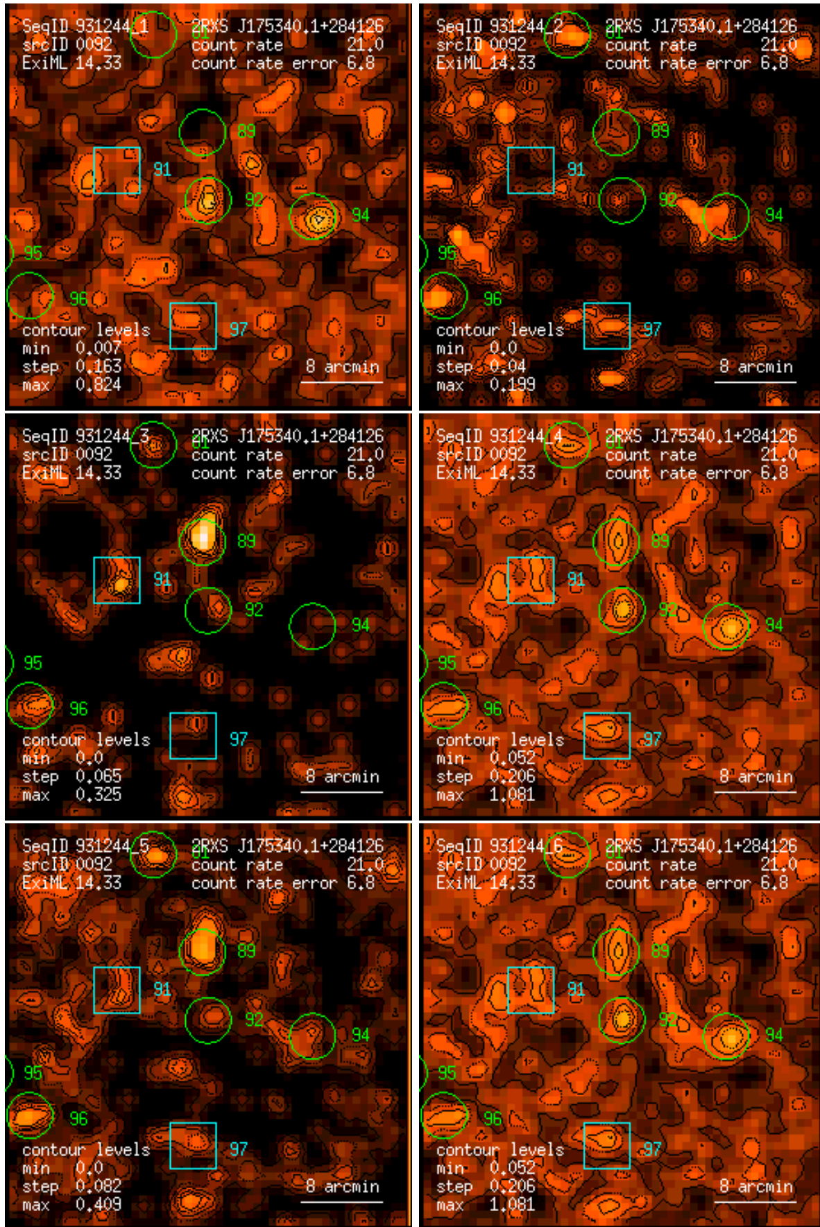
Figure 92: RASS 931244: detection 0092: band rate images, Gaussian filter: (1) PSPC channels 11 – 41, (2) 52 – 90, (3) 91 – 201, (4) 11 – 235, (5) 52 – 201, (6) 11 – 201. Broad band rates in counts/ks. Band rate contour levels in counts/ks/arcmin 2 .
