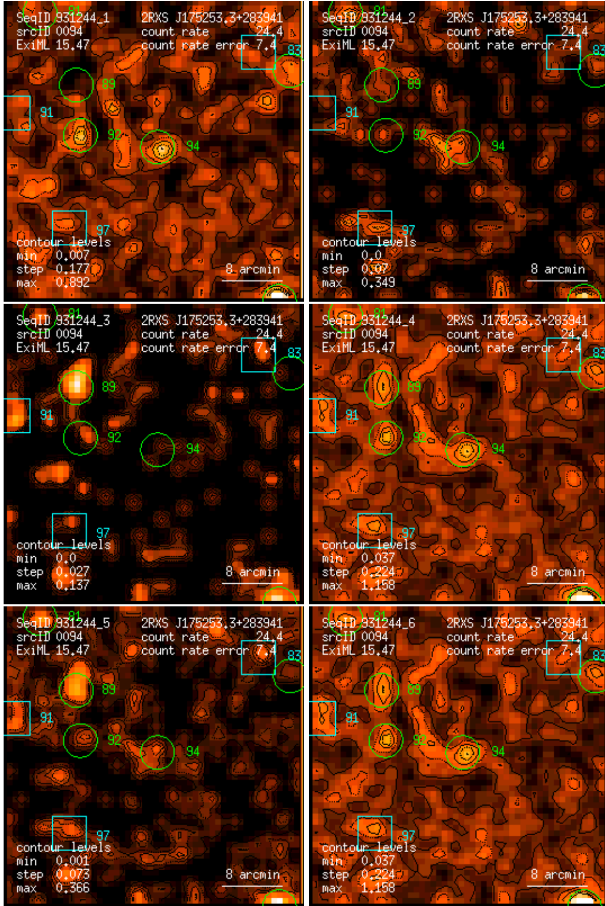
Figure 94: RASS 931244: detection 0094: band rate images, Gaussian filter: (1) PSPC channels 11 – 41, (2) 52 – 90, (3) 91 – 201, (4) 11 – 235, (5) 52 – 201, (6) 11 – 201. Broad band rates in counts/ks. Band rate contour levels in counts/ks/arcmin 2 .
