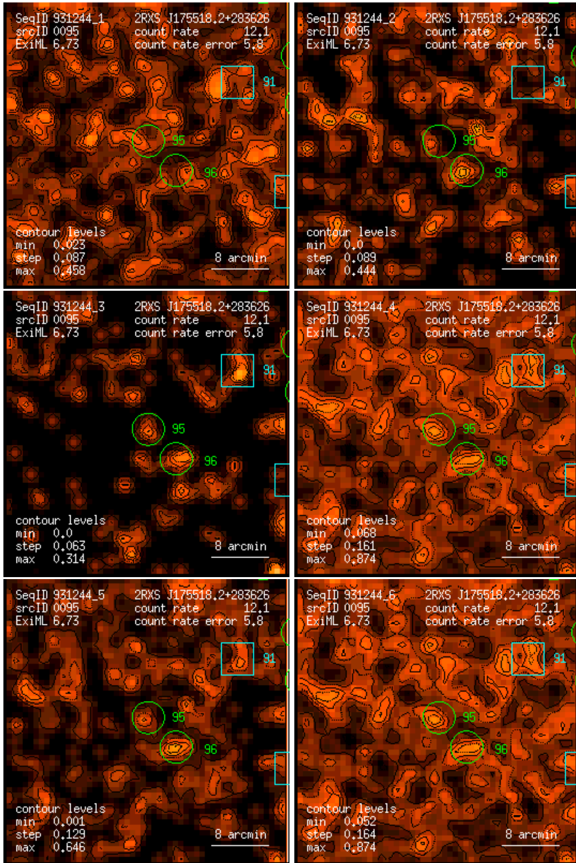
Figure 95: RASS 931244: detection 0095: band rate images, Gaussian filter: (1) PSPC channels 11 – 41, (2) 52 – 90, (3) 91 – 201, (4) 11 – 235, (5) 52 – 201, (6) 11 – 201. Broad band rates in counts/ks. Band rate contour levels in counts/ks/arcmin 2 .
