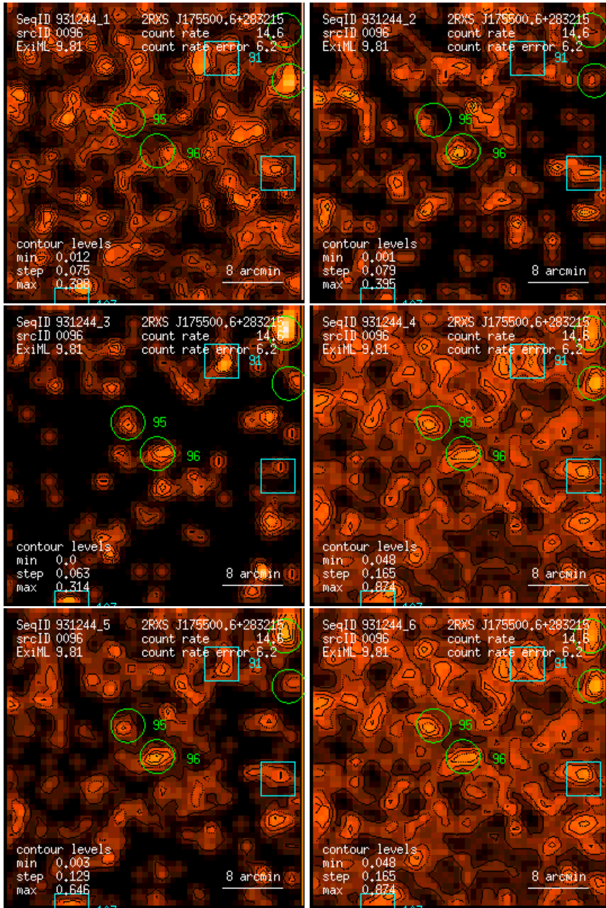
Figure 96: RASS 931244: detection 0096: band rate images, Gaussian filter: (1) PSPC channels 11 – 41, (2) 52 – 90, (3) 91 – 201, (4) 11 – 235, (5) 52 – 201, (6) 11 – 201. Broad band rates in counts/ks. Band rate contour levels in counts/ks/arcmin 2 .
