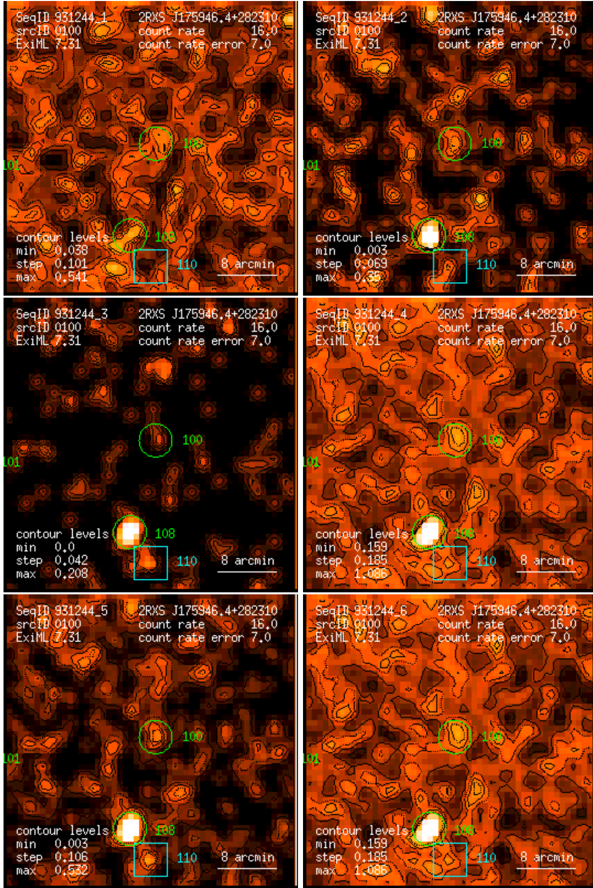
Figure 100: RASS 931244: detection 0100: band rate images, Gaussian filter: (1) PSPC channels 11 – 41, (2) 52 – 90, (3) 91 – 201, (4) 11 – 235, (5) 52 – 201, (6) 11 – 201. Broad band rates in counts/ks. Band rate contour levels in counts/ks/arcmin 2 .
