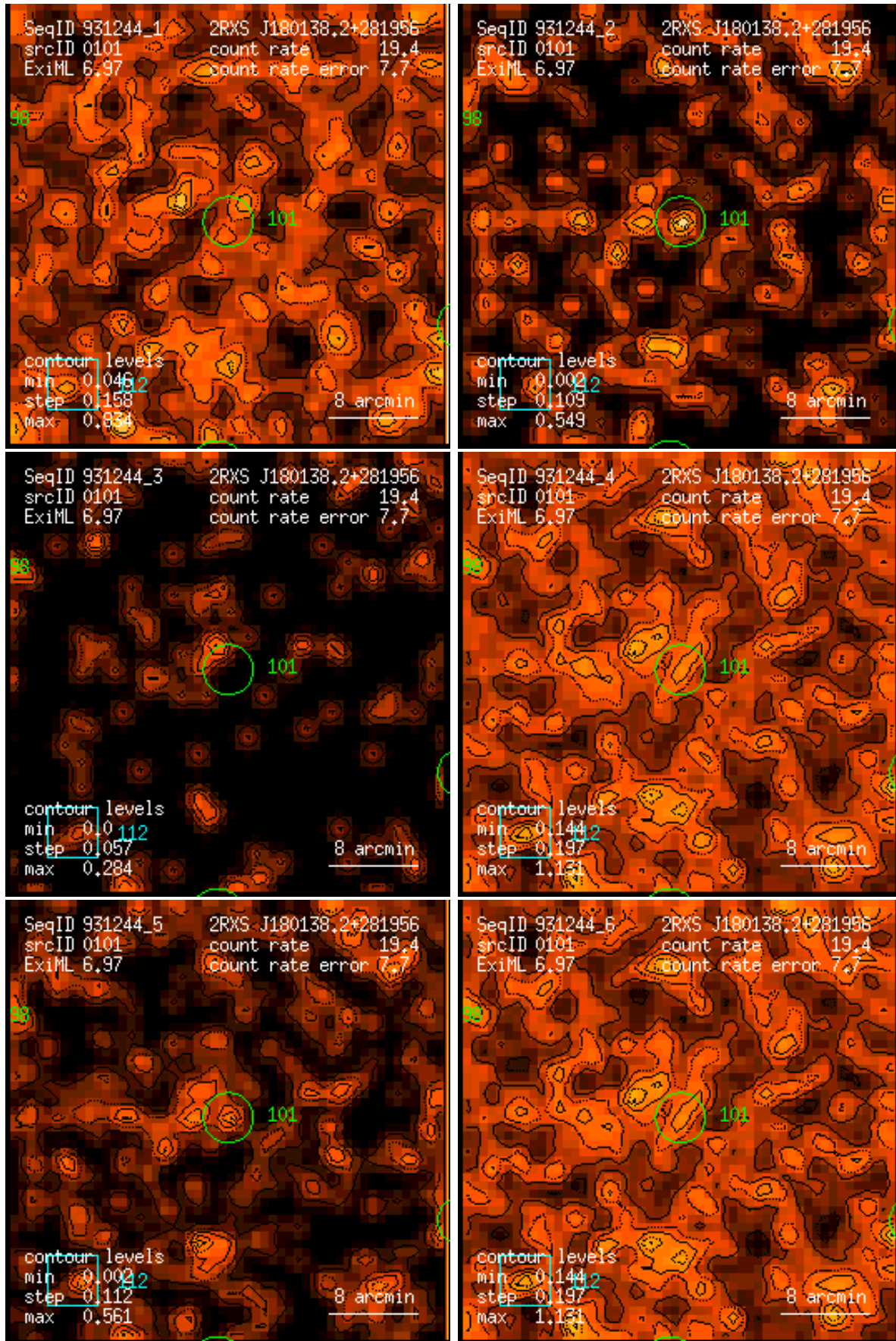
Figure 101: RASS 931244: detection 0101: band rate images, Gaussian filter: (1) PSPC channels 11 – 41, (2) 52 – 90, (3) 91 – 201, (4) 11 – 235, (5) 52 – 201, (6) 11 – 201. Broad band rates in counts/ks. Band rate contour levels in counts/ks/arcmin 2 .
