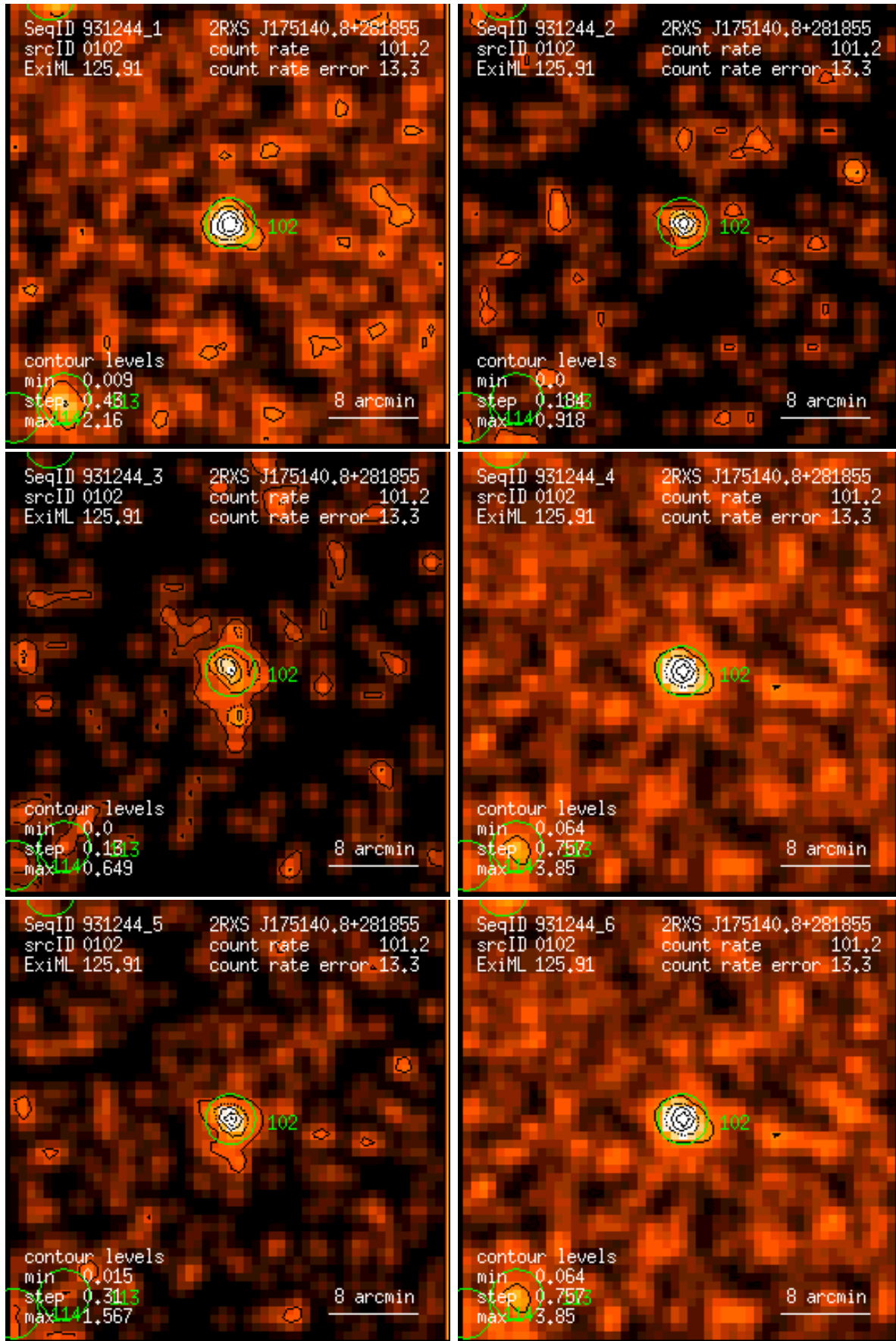
Figure 102: RASS 931244: detection 0102: band rate images, Gaussian filter: (1) PSPC channels 11 – 41, (2) 52 – 90, (3) 91 – 201, (4) 11 – 235, (5) 52 – 201, (6) 11 – 201. Broad band rates in counts/ks. Band rate contour levels in counts/ks/arcmin 2 .
