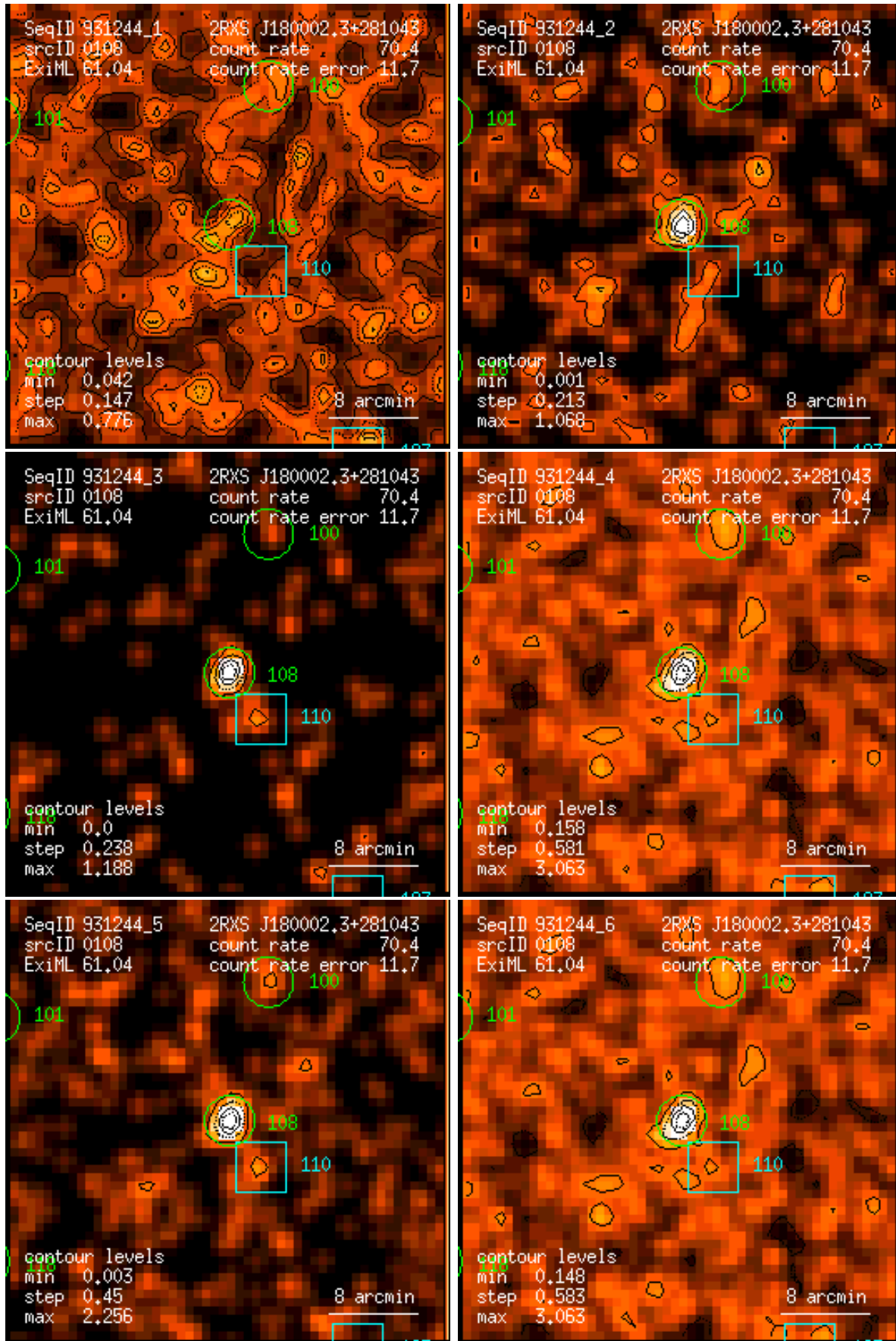
Figure 108: RASS 931244: detection 0108: band rate images, Gaussian filter: (1) PSPC channels 11 – 41, (2) 52 – 90, (3) 91 – 201, (4) 11 – 235, (5) 52 – 201, (6) 11 – 201. Broad band rates in counts/ks. Band rate contour levels in counts/ks/arcmin 2 .
