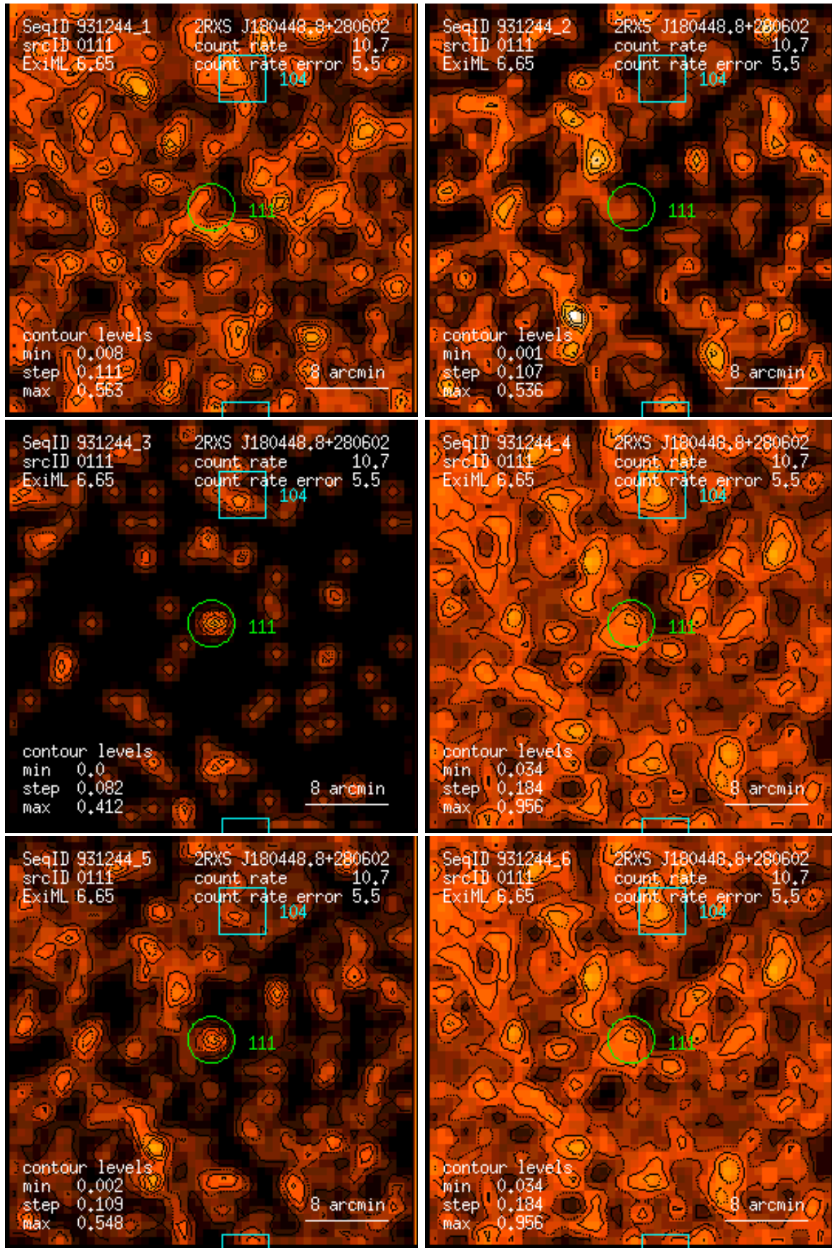
Figure 111: RASS 931244: detection 0111: band rate images, Gaussian filter: (1) PSPC channels 11 – 41, (2) 52 – 90, (3) 91 – 201, (4) 11 – 235, (5) 52 – 201, (6) 11 – 201. Broad band rates in counts/ks. Band rate contour levels in counts/ks/arcmin 2 .
