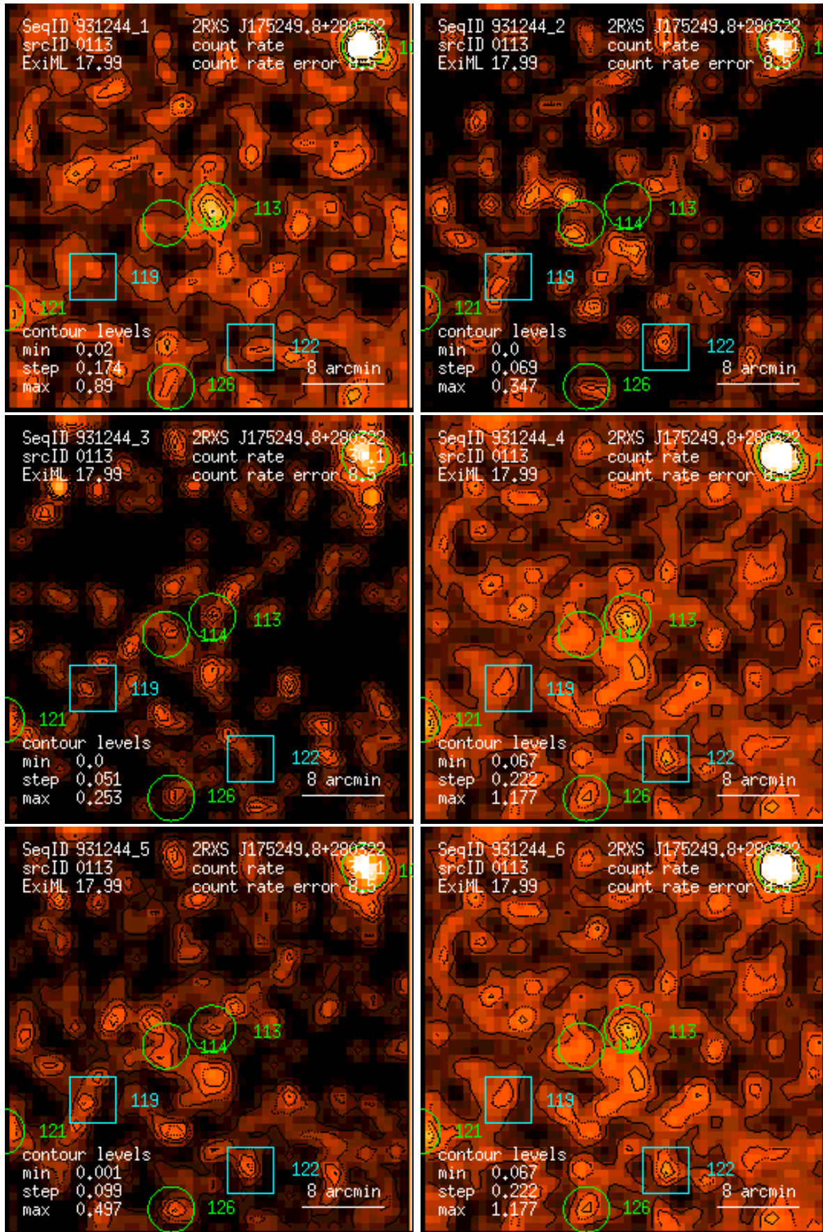
Figure 113: RASS 931244: detection 0113: band rate images, Gaussian filter: (1) PSPC channels 11 – 41, (2) 52 – 90, (3) 91 – 201, (4) 11 – 235, (5) 52 – 201, (6) 11 – 201. Broad band rates in counts/ks. Band rate contour levels in counts/ks/arcmin 2 .
