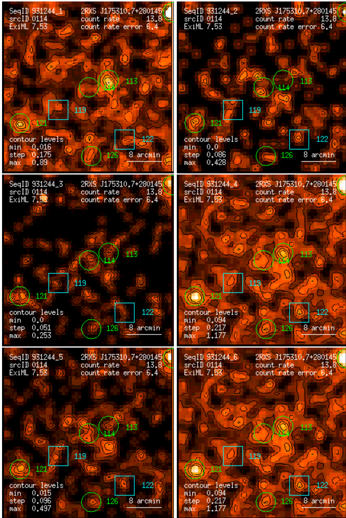
Figure 114: RASS 931244: detection 0114: band rate images, Gaussian filter: (1) PSPC channels 11 – 41, (2) 52 – 90, (3) 91 – 201, (4) 11 – 235, (5) 52 – 201, (6) 11 – 201. Broad band rates in counts/ks. Band rate contour levels in counts/ks/arcmin 2 .
