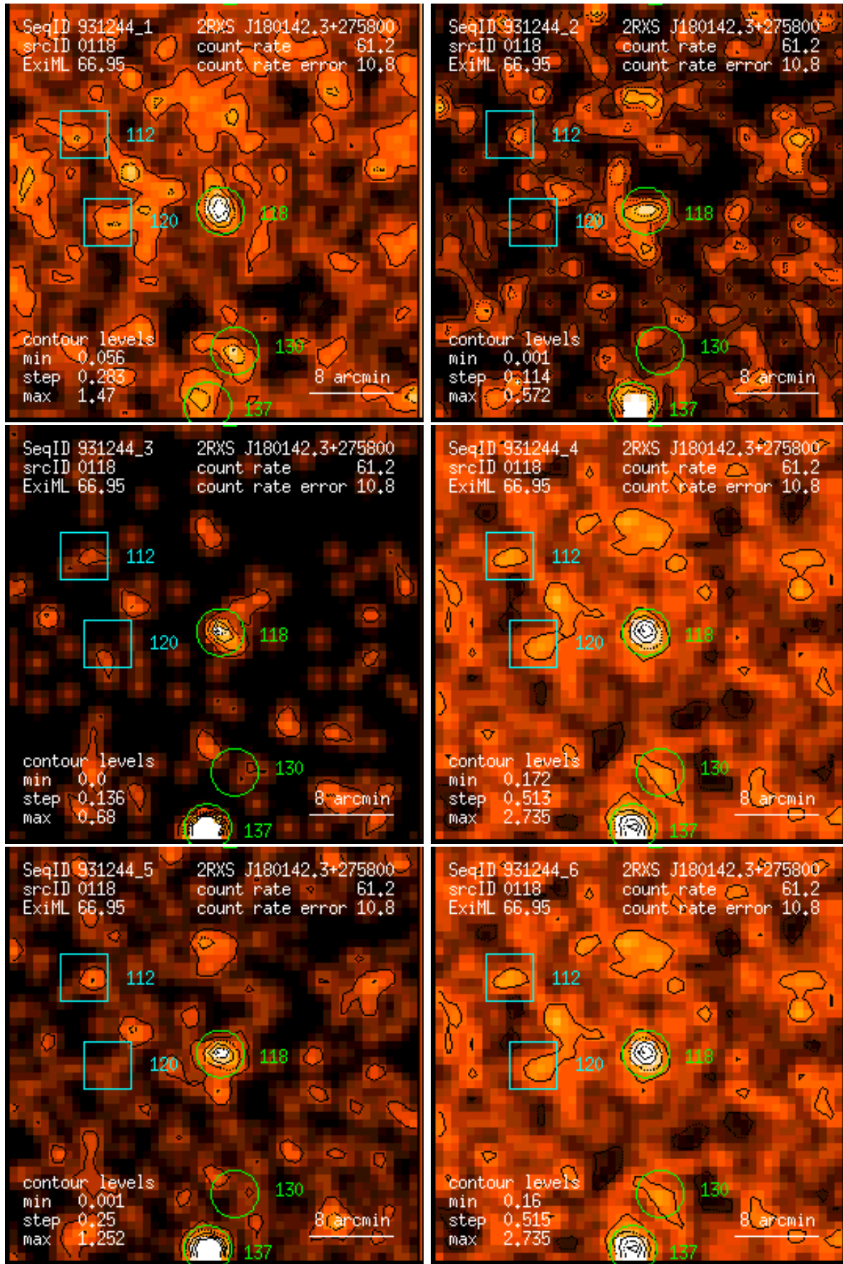
Figure 118: RASS 931244: detection 0118: band rate images, Gaussian filter: (1) PSPC channels 11 – 41, (2) 52 – 90, (3) 91 – 201, (4) 11 – 235, (5) 52 – 201, (6) 11 – 201. Broad band rates in counts/ks. Band rate contour levels in counts/ks/arcmin 2 .
